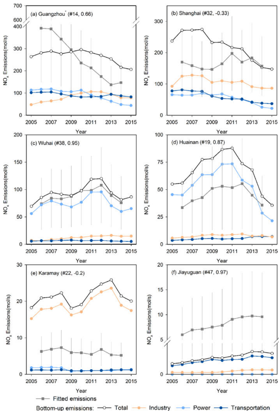
Figure 4. Interannual trends in the fitted (gray squares) and bottom-up anthropogenic NO x emissions for 2005 to 2015 including total (black circles), industrial (pink circles), power plant (light blue circles) and transportation (dark blue circles) emissions. Error bars denote the uncertainty of the fitted NO x emissions. The IDs from Fig. 1 and the correlation coefficients of the pair-wise trends between the bottom-up and fitted NO x emissions are shown in the bracket after the name of the city.
