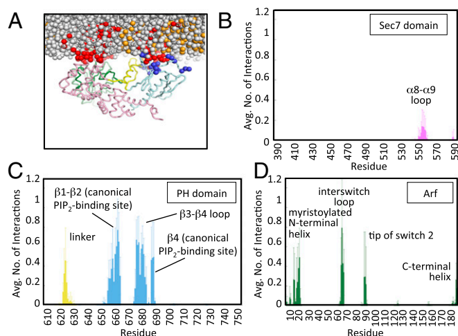
Fig. 3. Coarse-grained MD simulations of myr r Arf/Brag2 on a membrane showing multiple PIP 2 lipid-binding sites. (A) Close-up of myr r Arf/Brag2 at the end of the simulation run, for one run. Both myr r Arf and Brag2 bind primarily to PIP 2 molecules in the membrane at multiple binding sites. (B) Time-averaged number of interactions between Sec7 domain residues and PIP 2 lipids. (C) Time-averaged number of interactions between the linker and PH domain residues of Brag2 and PIP 2 lipids. (D) Time-averaged number of interactions between Arf residues and PIP 2 lipids. Color-coding for Brag2 and lipids is as in Figs. 1 and 2. Arf is in green.
