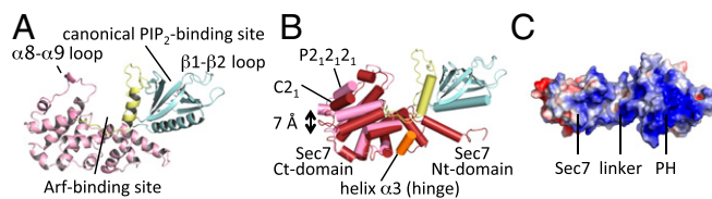
Fig. 1. Crystallographic analysis of uncomplexed Brag2. (A) Structure of unbound Brag2. Regions discussed in the text are indicated. The Sec7 domain is in pink, the linker in yellow, and the PH domain in blue. The same color scheme is used in all figures. (B) Overlay of Brag2 from P2 1 2 1 2 1 space group (light pink) and C2 1 space group (dark pink), showing the flexibility of the Sec7 C-terminal subdomain. The flexible hinge region is in orange. The orientation is as in A. (C) Electrostatic potential surface of unbound Brag2. The view is rotated by 90° with respect to A.
