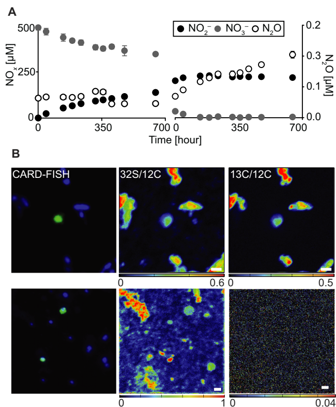
Fig. 3. Denitrifying potential of Nitrococcus mobilis Nb-231. (A) Anaerobic dissimilation under (left) organoheterotrophic conditions (500 \mu\text{M} ^{15}\text{NO}_3^- , 250 \mu\text{M} acetate, and 250 \mu\text{M} formate, anoxic) and (right) without the addition of electron donor (200 \mu\text{M} ^{15}\text{NO}_2^- , anoxic). See the main text for more details. Error bars indicate SD of three biological replicates. (B) FISH-SIMS analyses of single Nitrococcus cells in Namibian OMZ bottom water samples (1.20 m above seafloor), incubated with (top) ^{13}\text{C} -labeled dissolved organic matter (DOM) or (bottom) ^{13}\text{C} -labeled bicarbonate under hypoxic conditions. Left: Nitrococcus cells (green) targeted by CARD-FISH among other microbial cells (blue). Middle: ^{32}\text{S}/^{12}\text{C} of the corresponding cells. Right: ^{13}\text{C}/^{12}\text{C} ratio. Scale bars, 1 \mu\text{m} .
