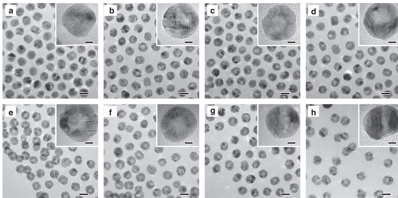
Fig. 3 TEM and HRTEM images of hollow Pd hollow nanocrystals obtained with varied molar ratios of N_2:O_2 : a 90:10, b 85:15, c 85:15, d 70:30, e 60:40, f 40:60, g 20:80, h 0:100. Scale bars are 20 nm. Scale bars in the insets are 5 nm
