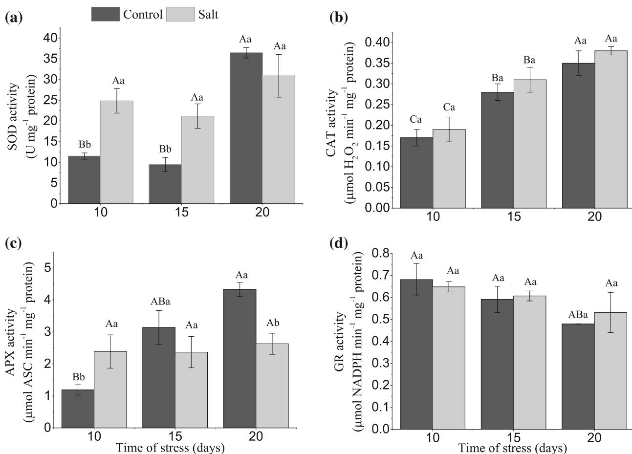
Fig. 2 Activity of the enzyme superoxide dismutase (a), catalase (b), ascorbate peroxidase (c), and glutathione reductase (d) in rice plants, cultivar BRS AG, subjected to salinity conditions at different times. Means of activity \pm SD ( n = 3 ), where uppercase letters indicate a
