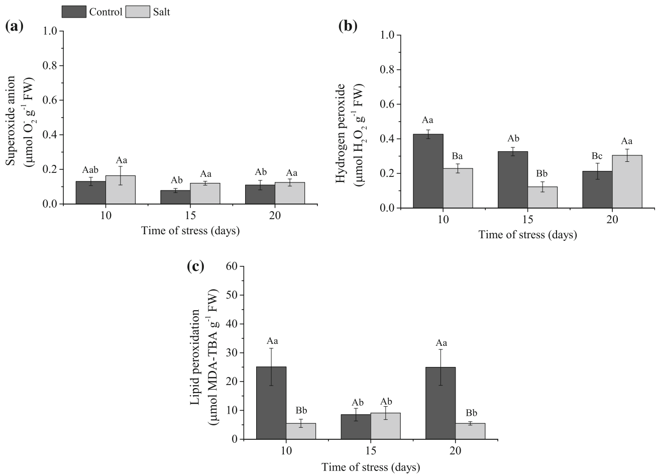
Fig. 1 Superoxide (a), hydrogen peroxide (b), lipid peroxidation (c) contents of rice plants, cultivar BRS AG, subjected to saline stress (136 mM). The values are represented by the mean of each treatment \pm SD ( n = 3 ). Uppercase letters indicate a significant
