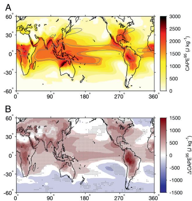
Fig. 1. (A) Ensemble mean of CAPE^{95} (colors) and 5 \text{ mm} \cdot \text{d}^{-1} contour of time mean and ensemble mean precipitation (gray) based on 12 CMIP5 models for the period 1981–2000. (B) Change in the ensemble mean CAPE^{95} from the current climate (1981–2000) to the future climate (2081–2100) under the RCP8.5 scenario. Stippling in B indicates regions where 11 of the 12 models agree on the sign of the response.
