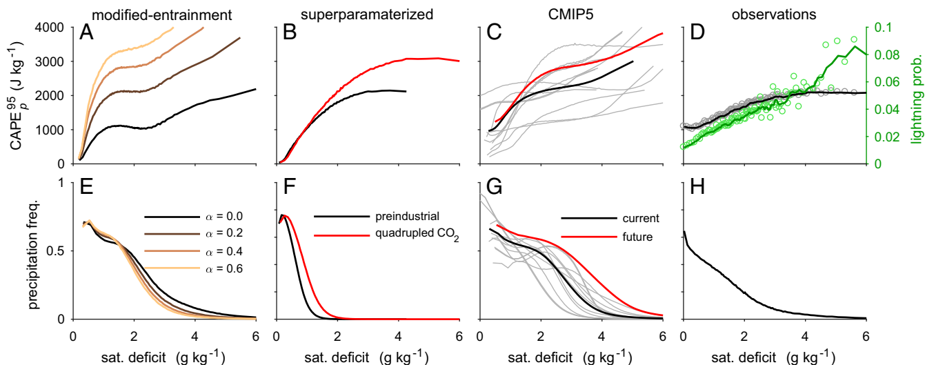
Fig. 3. (A–D) The 95th percentile of CAPE in strongly precipitating regions ( CAPE_p^{95} ; left axis) and (E–H) frequency (freq.) of daily precipitation exceeding 5 \text{ mm} \cdot \text{d}^{-1} , as a function of the lower-tropospheric saturation (sat.) deficit q_{\text{def}} for (A and E) modified entrainment simulations for different values of the entrainment parameter \alpha , (B and F) superparameterized GCM simulations of preindustrial climate (black) and quadrupled \text{CO}_2 concentration (red), (C and G) CMIP5 ensemble mean in the current climate (1981–2000; thick black; individual models shown in gray) and in the future climate under the RCP8.5 scenario (2081–2100; thick red), and (D and H) observations. Statistics are calculated using 100 bins, each containing roughly the same proportion of the available data. In D, lightning frequency in strongly precipitating regions is plotted as a function of lower-tropospheric saturation deficit (green, right axis), and lines are smoothed with a five-point Lowess filter, with symbols giving unsmoothed values.
