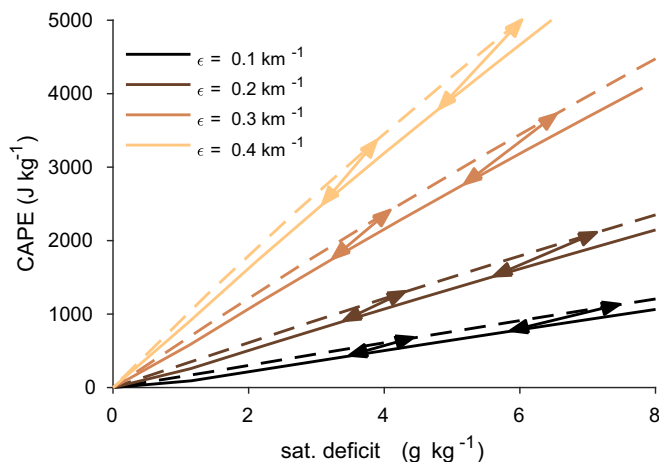
Fig. 4. CAPE as a function of lower-tropospheric saturation deficit q_{\text{def}} calculated using the zero-buoyancy plume model. Calculations are performed with a surface relative humidity of 80% and surface temperatures of 300 K (solid) and 303 K (dashed) for values of the environmental relative humidity in the free troposphere varying between 20% and 100% and entrainment rates \epsilon as given in the legend. Arrows connect solutions with the same relative humidity for different surface temperatures.
