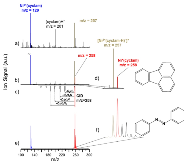
Figure 2. QIT mass spectra of (a) \text{Ni}^{2+}(\text{cyclam}) at m/z = 129 and (b) the ETD reaction of isolated monoisotopic \text{Ni}^{2+}(\text{cyclam}) with fluoranthene (top structure), which shows a peak corresponding to the formation of \text{Ni}^+(\text{cyclam}) at m/z = 258. Trace d expands the crucial region of trace b. CID on m/z = 258 results in the mass spectrum in trace c. Traces e and f show the analogous reaction of \text{Ni}^{2+}(\text{cyclam}) with the azobenzene anion (bottom structure).
