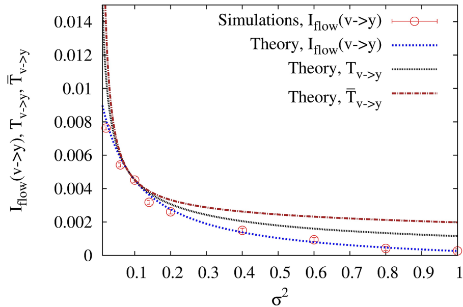
Fig 6. \mathcal{T}_{v \rightarrow y} , \bar{\mathcal{T}}_{v \rightarrow y} and \mathcal{I}_{v \rightarrow y}^{flow} as a function of the noise intensity \sigma^2 . The parameters of the model are T = 5 , \gamma = m = 1 , \tau_r = 0.1 and a = -0.7 .
