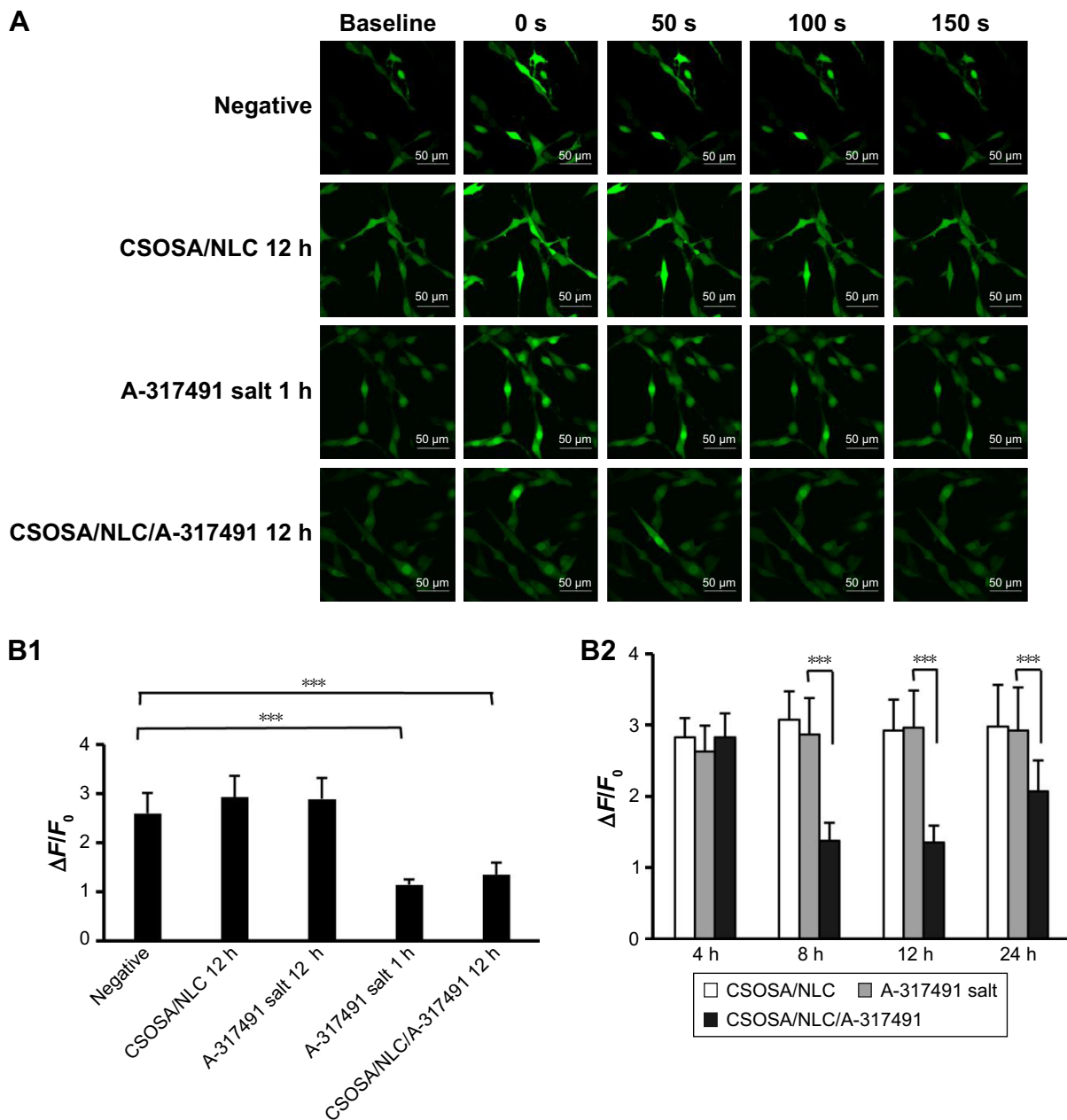
Figure 4 Inhibition of ATP-induced Ca 2+ influx in PC12 cells.
