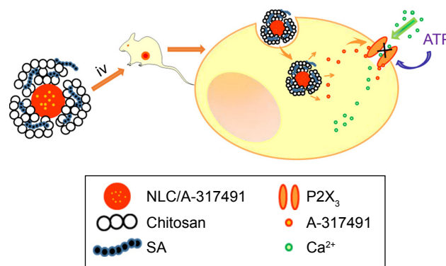
Figure 8 Schematic structure of CSOSA/NLC/A-317491 and its inhibition of ATP-induced Ca^{2+} influx.
