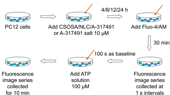
Figure 1 The methodology of intracellular calcium measurements.
