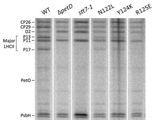
Fig. 3. Subunit IV fg loop mutants show low levels of Stt7-dependent LHCII phosphorylation. Autoradiogram of in vivo ^{32} P-labeled thylakoid polypeptides, extracted from cells placed in reducing conditions (5 \mu M FCCP, dark, 30 min) and separated by SDS/PAGE on an 8 M urea 12–18% gradient gel.
