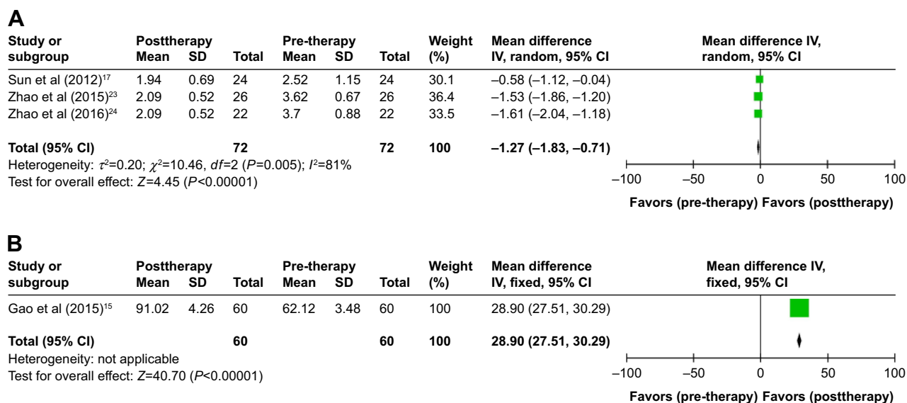
Figure 5 Forest plot of the comparison of Ps (A) score and Kps (B) in pre- and posttherapy.
