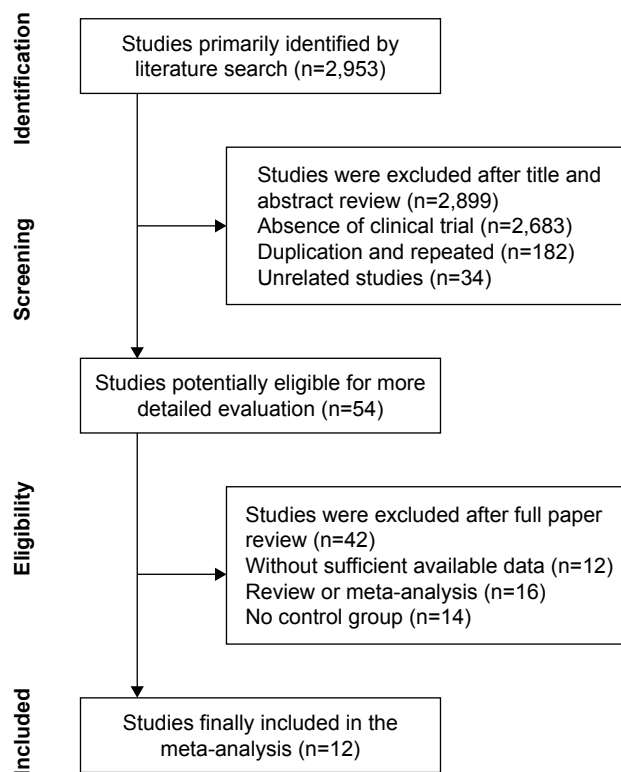
Figure 1 Flow diagram of the selection process.
