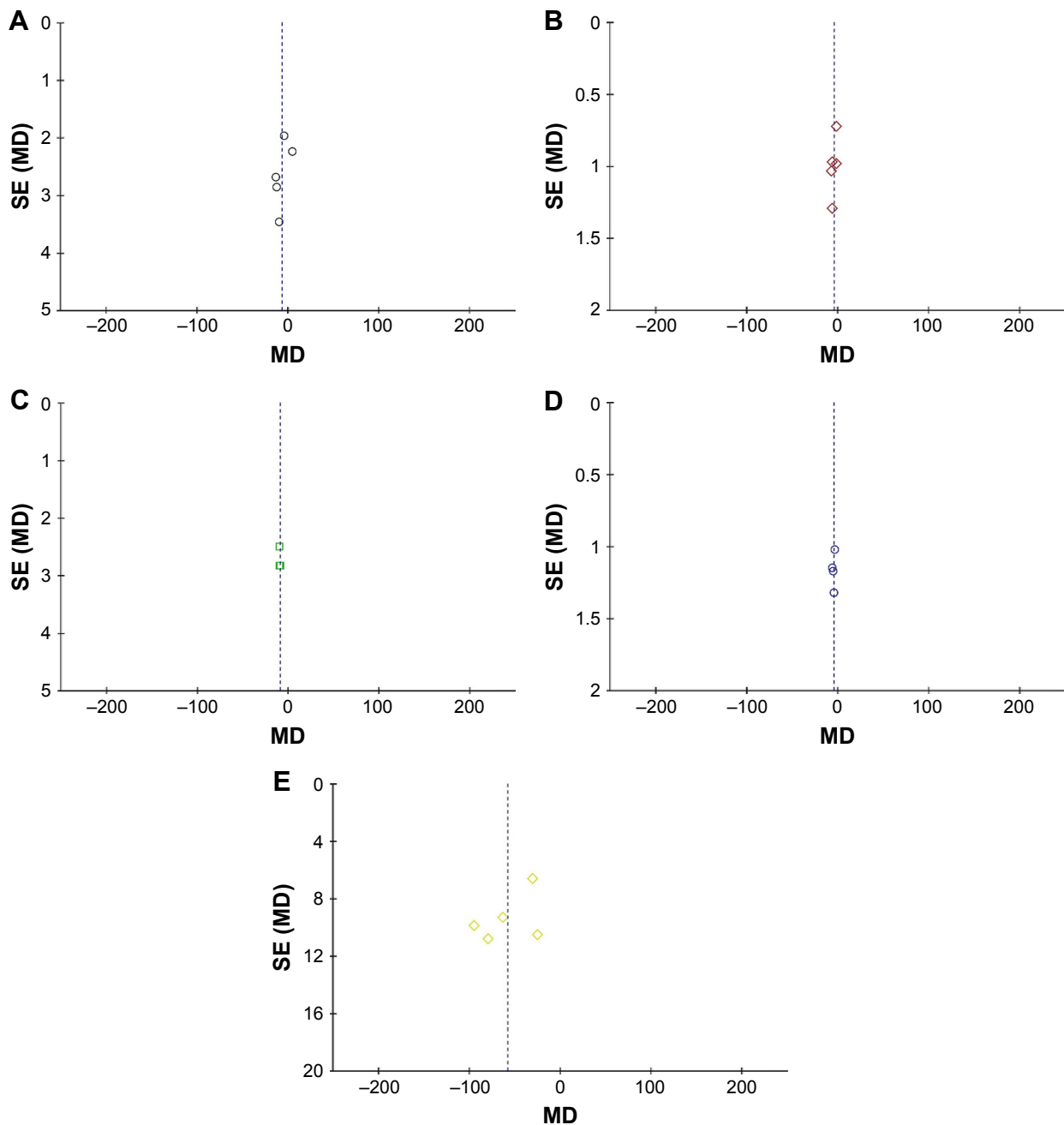
Figure 4 Funnel plot of percentage of tumor cells (A), serum level of \beta 2-M (B), serum level of M protein (C), 24 h urine light chain content (D), and Scr level (E). Abbreviations: \beta 2-M, \beta 2-microglobulin; MD, mean difference; Scr, serum creatinine; SE, standard error.
