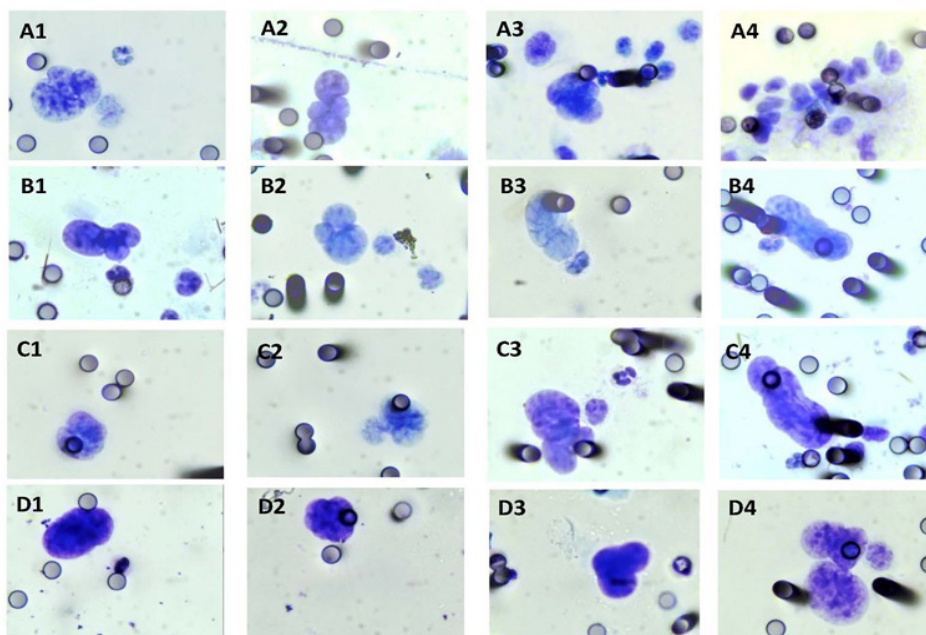
Figure 2. Histo-Pathological/ Cyto-Morphological Detection of CTC Using the ISET Method. CTC are stained blue, filter pores of 8 microns appear black. Panel A: breast cancer, B: prostate cancer, C: colorectal cancer, D: renal/ bladder cancer
