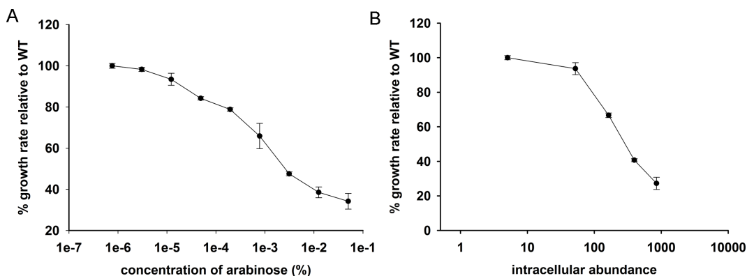
Figure 1. Representative gene-dosage toxicity curves for E. coli Dihydrofolate Reductase (DHFR) expressed from pBAD-plasmid (Bhattacharyya et al. , 2016). A. Plot of relative growth
