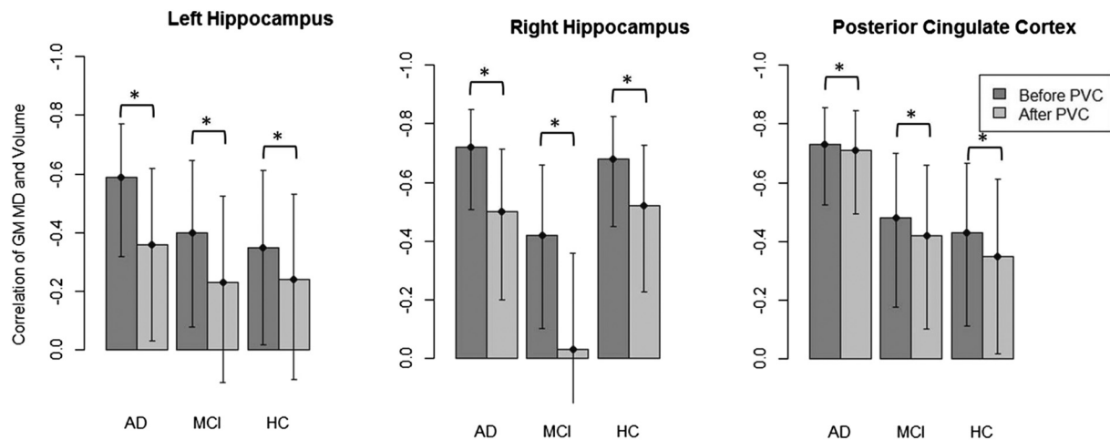
Fig. 3. Partial correlations of uncorrected and corrected GM MD values with GM volume, controlled for MRI protocol, age, gender and years of education. The bars on the left always represent the MD values without PVC, bars on the right represent MD values with PVC. *indicates significant differences of the partial correlations according to the Williams' test, error bars show confidence intervals (95%) of correlation coefficients.
