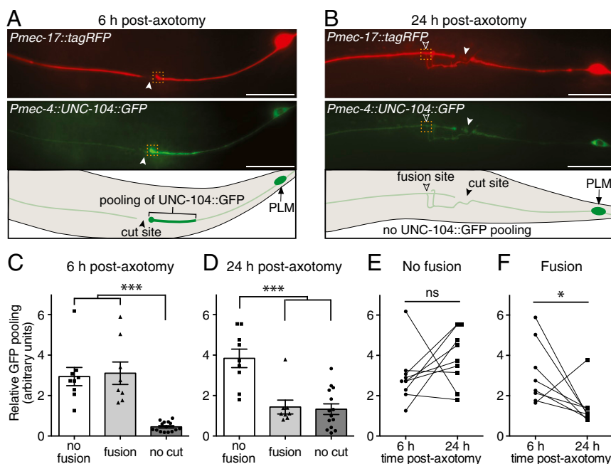
Fig. 2. Axonal transport is restored after axonal fusion. (A) Images and schematic 6 h after axotomy of PLM expressing diffusible tagRFP and UNC-104::GFP. Transection of the PLM axon prevents the normal anterograde transport, leading to pooling of UNC-104::GFP fluorescence on the proximal side of the cut site. Closed arrowheads designate cut sites. (Scale bars: 25 \mu\text{m} .) (B) By 24 h postaxotomy, axonal fusion has occurred in the same animal as shown in A, restoring axonal transport and releasing the pool of UNC-104::GFP. Open arrowheads designate fusion sites; dashed boxes in A and B highlight the regions used for quantification of relative GFP pooling in C–F. (C and D) Quantification of GFP pooling at 6 (C) and 24 h (D) postaxotomy in animals that regrew without axonal fusion (no fusion) (Fig. S2B and C), those that displayed fusion, and those in which no axotomy was performed (no cut). Bars represent mean \pm SE. Symbols represent individual animals; n \geq 8 . P values are from Tukey's multiple comparisons test. *** P < 0.001 . Comparison of relative GFP pooling levels at 6 and 24 h postaxotomy (E) in animals where axonal fusion was not observed and (F) in animals where fusion was observed. Data shown in E and F are replotted from C and D. Symbols represent individual animals, and lines connect the responses of the same animals; P values are from paired t tests. ns, not significant. * P < 0.05 .
