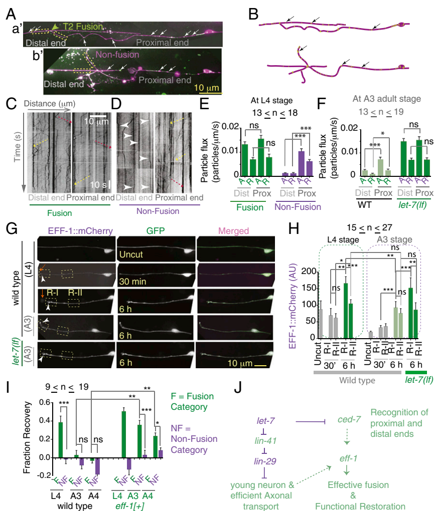
Fig. 6. Loss of let-7 improves axonal transport during axonal fusion. (A, a' and b') Still images from time-lapse movies of the PLM with tbs222 ( Pmec-4 -mCherry) and jsIs821 ( Pmec-7 -GFP::RAB-3) using spinning-disk confocal at 24 h postaxotomy. mCherry is shown in magenta, and GFP::RAB-3 is shown in green. White arrows indicate GFP::RAB-3 particles in the axon. (A, a') T2 fusion. (A, b') Nonfusion. (B) Schematic representation of images shown in A. (C) Kymographs from the movies of 180-s duration were generated from the 30-μm ROIs (yellow dotted box in A, a') placed on the distal and proximal ends of fused neuron. Diagonal tracks represent events of anterograde (dashed yellow arrow) or retrograde (dashed red arrow) movements. (D) A kymograph from the distal and proximal ends of a nonfused axon as shown in A, b'. The perpendicular tracks (arrowheads) represent static particles. (E) The bar chart represents particle flux in the proximal and distal ends measured in fusion and nonfusion events. A, anterograde events; R, retrograde events. Particle flux = number of particles or tracks per micrometer per second. N = 5-8 independent replicates. (F) The bar chart shows flux values in the proximal and distal ends in A3 worms measured in T2 fusion events. N = 4-7 independent replicates. (G) Spinning-disk confocal images of worms coexpressing muls32 ( Pmec-7 -GFP) and shrEx59 ( Pmec-4 -EFF-1::mCherry) before and after axotomy. Orange arrows indicate the site of axotomy. Two ROIs are shown: R-I at the cut tip and R-II placed 10 μm away from ROI-I to quantify the average intensity of EFF-1::mCherry. EFF-1 intensity is increased at R-I at 6 h after axotomy. This enrichment is reduced at the A3 stage. (H) The average intensity of EFF-1::mCherry in two ROIs obtained 30 min before and 6 h after axotomy is plotted for L4- and A3-stage experiments. N = 2-4 independent replicates. (I) In the eff-1(+) strain shrEx59 ( Pmec-4 -EFF-1::mCherry), FR values in the fusion category are increased significantly compared with the values in wild-type strain at the A3 and A4 stages. N = 2 . In E, F, H, and I, * P < 0.01 ; ** P < 0.001 ; *** P < 0.0001 ; ANOVA with Newman-Keuls multiple comparisons test. Error bars represent SEM. (J) The working model depicting how the let-7 miRNA pathway negatively regulates effective axon fusion in L4 and aged worms. ns, not significant.
