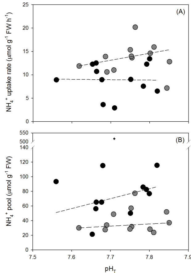
Fig 3. (A) \text{NH}_4^+ uptake rates ( \mu\text{mol g}^{-1} \text{FW hour}^{-1} ) in 20 \mu\text{M} \text{NH}_4^+ seawater for 30 minutes and (B) internal \text{NH}_4^+ pools ( \mu\text{mol g}^{-1} \text{FW} ) for Ulva australis grown under ambient and enriched \text{NH}_4^+ treatments across a range of \text{pH}_T s. Grey points represent ambient \text{NH}_4^+ treatments and black points represent enriched \text{NH}_4^+ treatments. A plus symbol (+) indicates an outlier which was removed for statistical analysis. The slopes of \text{NH}_4^+ uptake rates and internal \text{NH}_4^+ pools with \text{pH}_T for each \text{NH}_4^+ treatment (dashed lines) were tested for an interaction using an ANCOVA.
