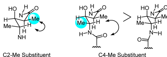
Figure 13. C2 and C4 methyl groups of the valerate linker in bleomycin induce a rigid, compact versus extended conformation productive for DNA cleavage; see Figure 12. Each heavy atom substituent independently increases the efficiency of DNA cleavage without impacting metal chelation, O 2 activation, or the cleavage reaction and without making direct contact with the target.
