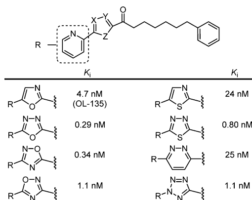
Figure 15. Representative OL-135 analogues containing iterative single heavy atom changes or exchanges in the activating heterocycle. Reduction in the steric size of the heterocycle position 4 heavy atom (potency: N > O > CH ) contributes to increased inhibitor potency.
