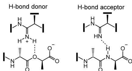
Figure 2. Vancomycin analogues that incorporate single heavy atom changes in the binding pocket.
