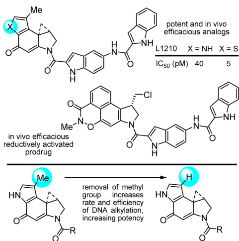
Figure 11. Additional simplifying structural modifications, an example of removal of a single heavy atom (Me group) that improves potency by making the underlying DNA alkylation reaction sterically more accessible, and a recent efficacious prodrug design on a simplified structure.
