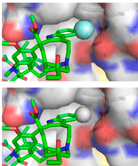
Figure 6. Model of the 10'-fluoro binding site of 10'-fluorovinblastine ( R = F , top) generated by adding the fluorine substituent to the X-ray structure of tubulin-bound vinblastine 67 ( R = H , bottom). 64 Modeled complexes with larger substituents ( R = Cl, Me, Br, I ) exhibited increasingly larger destabilizing steric interactions as the substituent size progressively increased.
