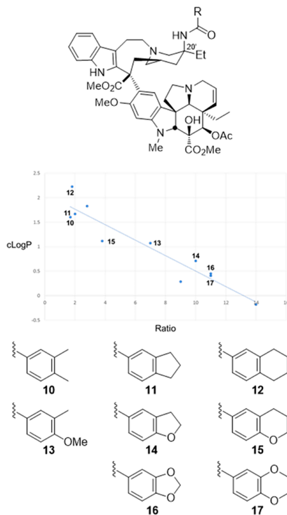
Figure 8. Plot of 20' amide cLogP versus differential activity ( IC_{50} ratio) for isogenic HCT116 resistant (Pgp overexpression) and sensitive cell lines that progressively exchange in single heavy atoms or heteroatoms. The correlation defines a linear relationship between diminished resistance (ratio) that arises from reduced/abolished Pgp efflux, and a modulated physical property of the compounds (lipophilic character, cLogP) that can be predictably impacted by single atom changes. All compounds shown are more potent than vinblastine and display less resistance (vinblastine ratio = 88).
