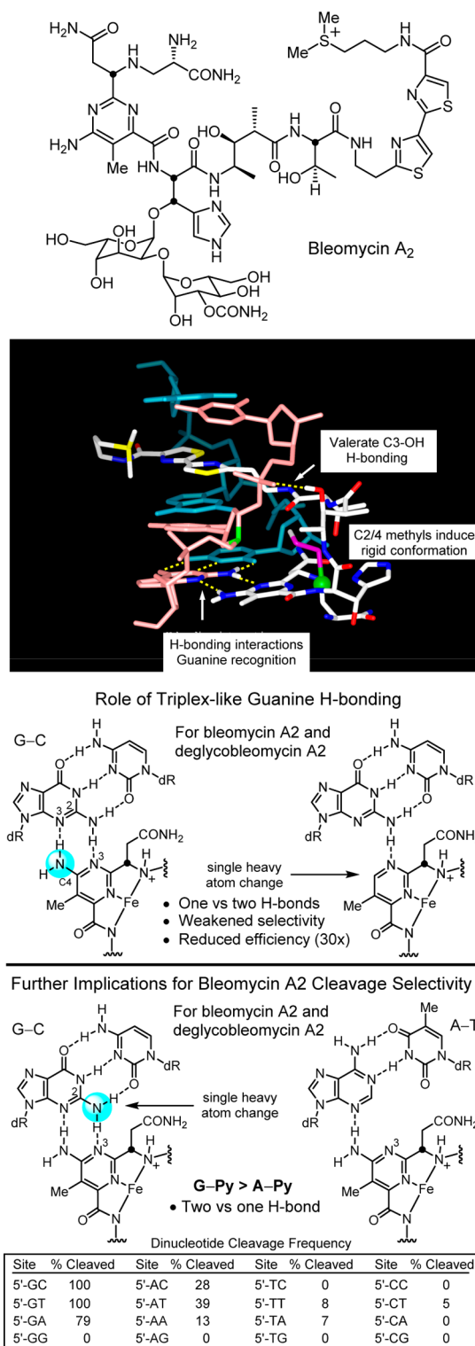
Figure 12. Structure of bleomycin A 2 , NMR structure of bleomycin bound to a DNA cleavage site (full deoxyoligonucleotide and bleomycin disaccharide removed for clarity), key H-bonding role the pyrimidine C4 amine plays in guanine recognition, and role the minor groove guanine C2 amine plays in the recognition of bleomycin.
