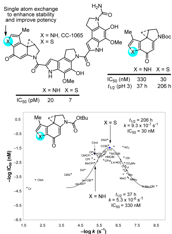
Figure 10. Single heavy atom exchange in the CC-1065 alkylation subunit that improves potency through a predictable reduction in intrinsic reactivity, placing it at an optimal point on a parabolic relationship between functional reactivity and activity.
