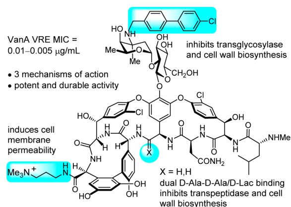
Figure 3. Vancomycin analogue that contains a single atom change in the binding pocket, reinstating activity against vancomycin-resistant bacteria, and two peripheral modifications that add two additional independent mechanisms of action.
