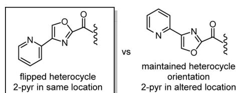
Figure 17. Superimposition of the X-ray structures of OL-135 (green) and its isomer (blue) bound to FAAH that illustrates the compensating impact of exchanging the location of two complementary heteroatoms.
