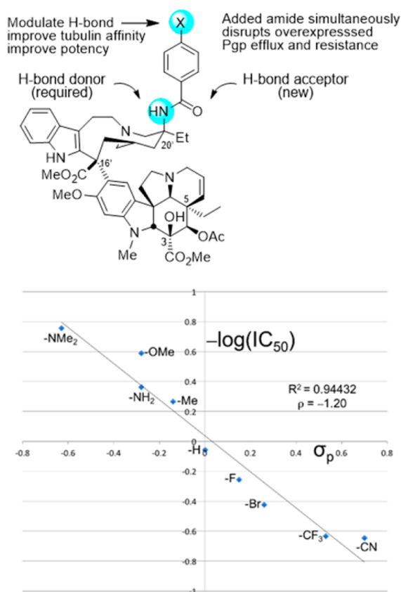
Figure 7. Active analogues required a single heavy atom exchange into the vinblastine structure (C20' NH 2 for OH). In a plot of -\log IC_{50} (nM, HCT116) versus substituent \sigma_p , the analogues additionally displayed a predictable modulation of activity by a substituent (X) electronic effect, impacting benzamide carbonyl H-bonding with tubulin, some representing single heavy atom additions. All analogues shown are more active than vinblastine.
