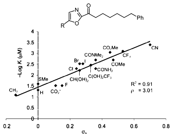
Figure 16. -\log K_i ( \mu\text{M} ) for FAAH versus Hammett \sigma_p , defining and quantitating a linear correlation between enzyme inhibition and the electronic impact of oxazole substituents on intrinsic reactivity of the electrophilic carbonyl of an \alpha -keto heterocycle ( \rho = 3.0 ), some arising from single heavy atom substitution.
