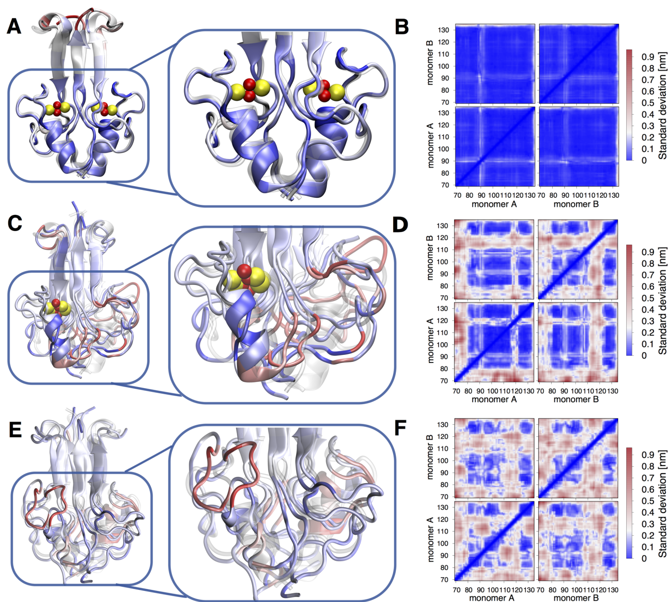
Figure 2. Structure and conformational fluctuations of NAF-1 (A, B), semi-holo NAF-1 (C, D), and apo NAF-1 (E, F). (A, C, E) Superimposition of the X-ray structures (transparent) with several MD representatives, color coded as follows: blue: relatively rigid structure, PAD < 20^\circ ; white: low flexibility, 20^\circ < PAD < 80^\circ ; red: high flexibility, PAD > 80^\circ . (B, D, F) Standard deviation matrices of the three proteins. (C) The [2Fe-2S] cluster has been removed from monomer “B”. (F) A loss of off-diagonal blue squares pattern points to a partial unfolding of \beta -sheets (aa 84–88; 94–98; 128–132).
