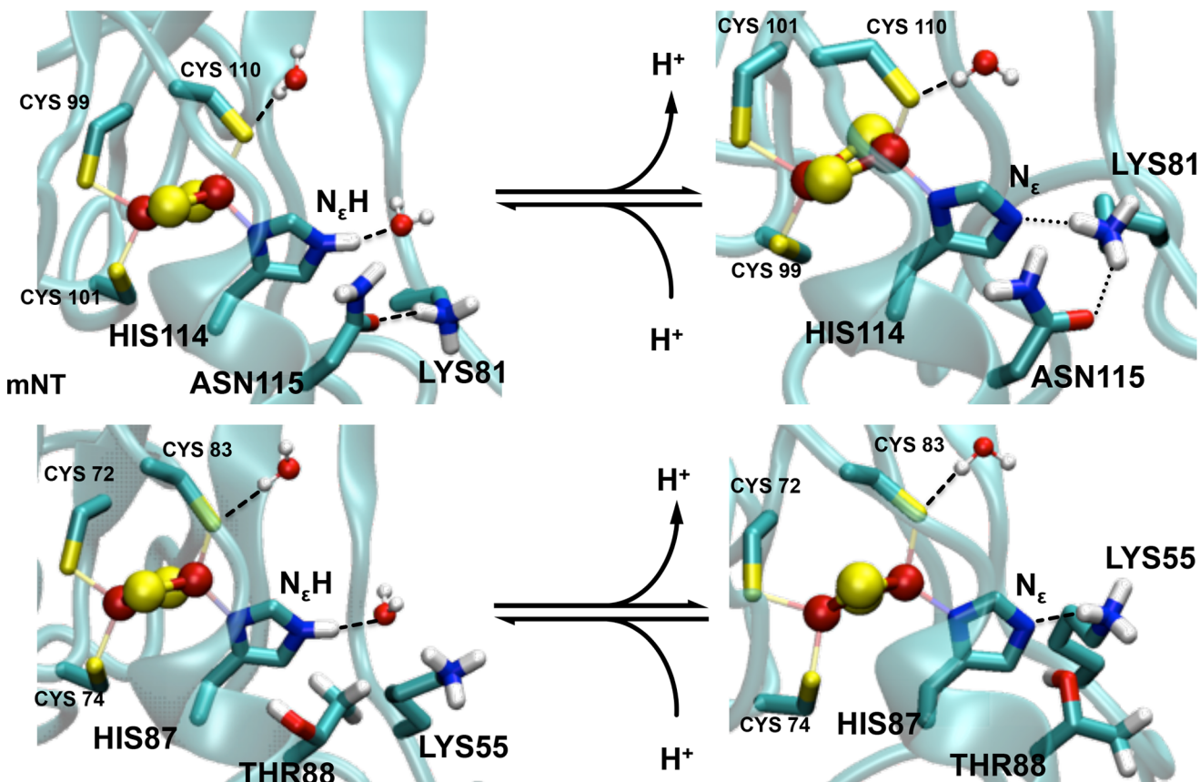
Figure 4. Histidine hydration in NAF-1 (A) and mNT (B). The protonated histidine ligand forms a H-bond with water molecule. The deprotonated histidine residue forms an H-bond with a lysine side chain or with water (not shown). The lysine forms an additional H-bond with a residue close by the cluster (Asn115) in NAF-1, but it can do so neither with the equivalent structural position (Thr88) nor with other residues nearby the cluster.
