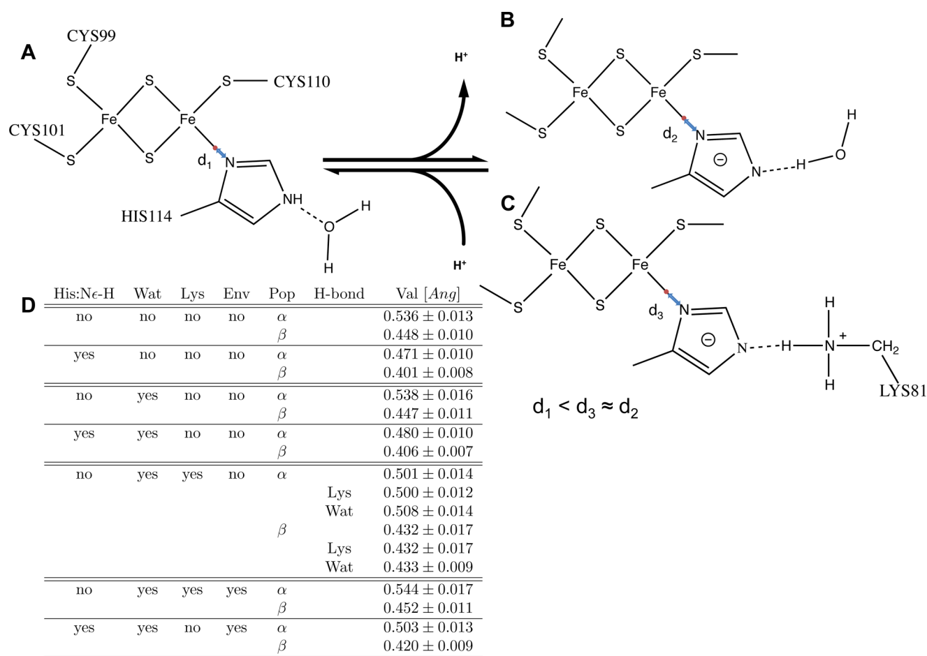
Figure 3. His: N_{\delta} -Fe bond polarity in NAF-1. It is estimated from the distance between N_{\delta} and BOCs, as obtained by spin-polarized DFT calculations (see Section 2.3). His114: N_{\epsilon} forms an H-bond with either water (B) or Lys81 (C), whereas His114: N_{\delta} -H forms H-bond only with water (A). Table (D) contains the BOCs distances from N_{\delta} (Val) in the presence (yes) and the absence (no) of coordinating histidine N_{\epsilon} proton (His: N_{\epsilon} -H), nearest water molecules to the coordinating sites (Wat), Lys81 (Lys), and protein environment (Env). The distances are reported for both \alpha and \beta electron populations (Pop). The H-bond column (where specified) indicates the H-bonding partner (Lys81 or water) of the N_{\epsilon} .
