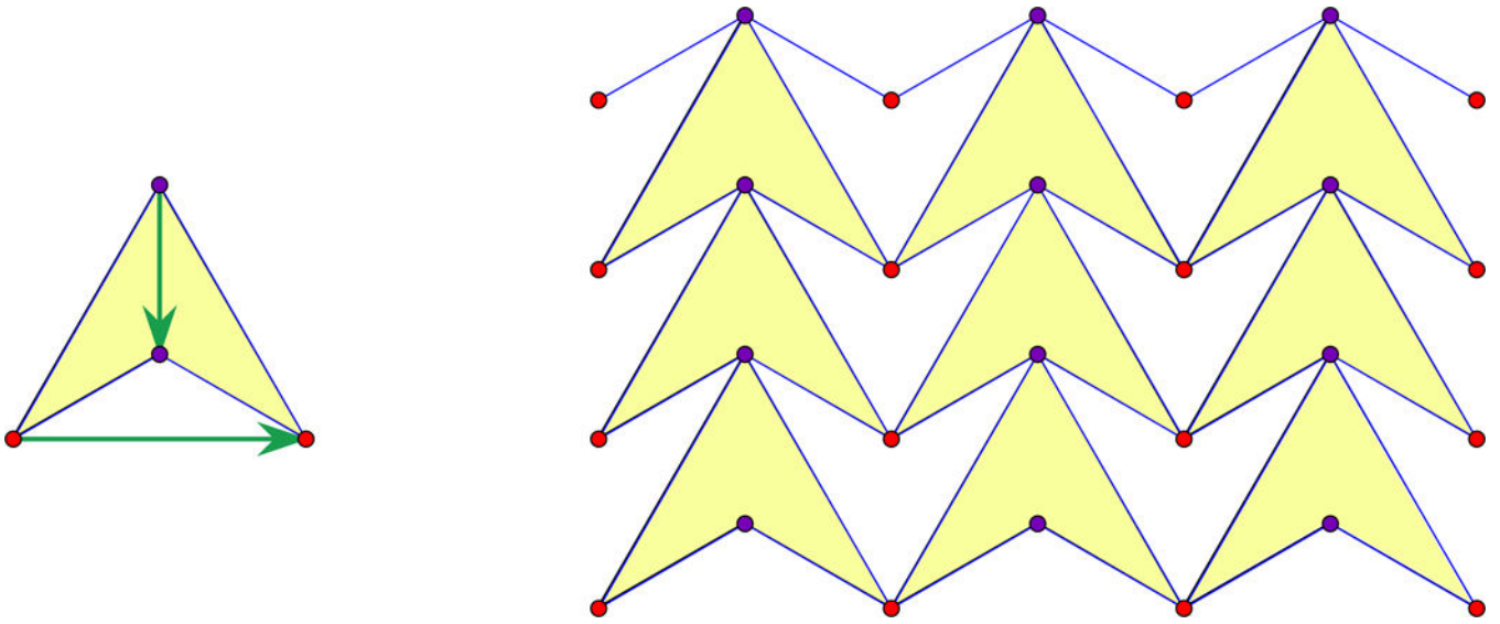
Figure 2. A planar four-bar mechanism with two marked pairs of vertices and the associated “double arrowhead” periodic framework.
