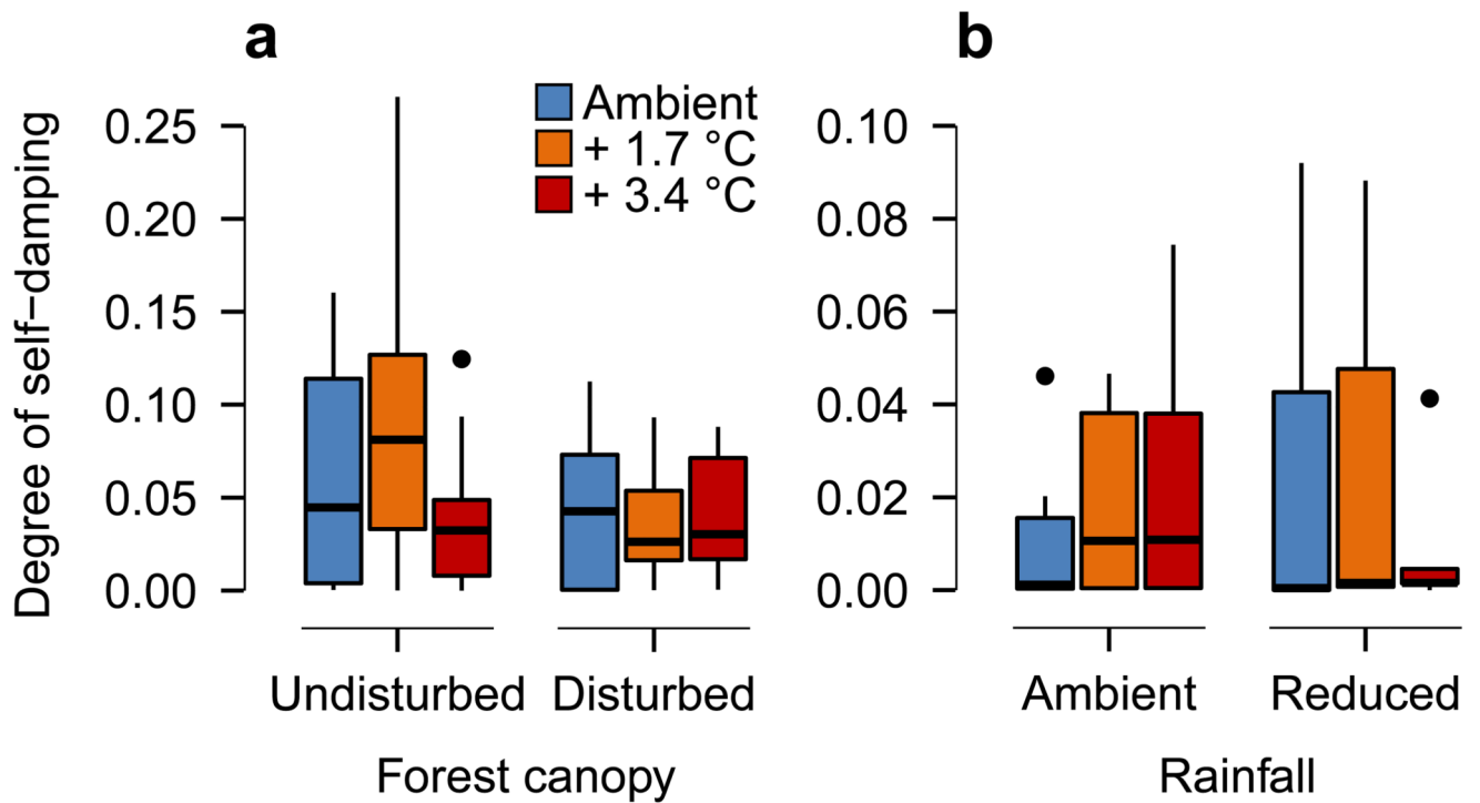
Figure 3. Effects of warming, canopy disturbance, and drought on whole network resilience. Presented are treatment effects in (a) the first (n=69) and (b) the second experiment (n=34) on the degree of self-damping (minimum s ) that is required for all eigenvalues of the Jacobian matrix to have negative real parts. Food webs that required a smaller degree of self-damping were considered to be more resilient to perturbations. Here, differences among treatments are not significant. Box plots are based on median (horizontal line), first and third quartile (rectangle), 1.5 \times interquartile range (whiskers), and outliers (isolated points).
