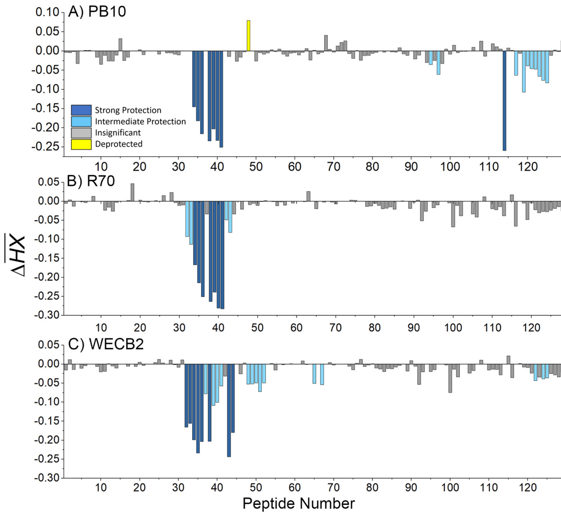
FIG 3 Relative levels of protection of RiVax peptides by PB10, R70, and WECB2, as defined by HX-MS. RiVax was subjected to HX-MS analysis in the presence of (A) PB10, (B) R70, and (C) WECB2. The \Delta HX values for each RiVax peptide are shown and colored according to their k -means categorization as follows: strong protection, deep blue; intermediate protection, light blue; insignificant protection, gray; deprotection, yellow.
