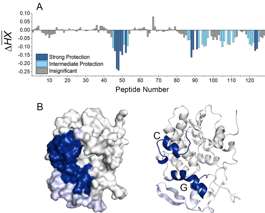
FIG 7 Localization of the core epitope of IB2 on RiVax. (A) The \overline{\Delta HX} values for each RiVax peptide shown for IB2 are indicated and are color coded according to the Fig. 3 legend. (B) The HX protection categories, as defined for panel A, are shown mapped onto the structure of RiVax. The locations of \alpha -helices C and G are indicated.
