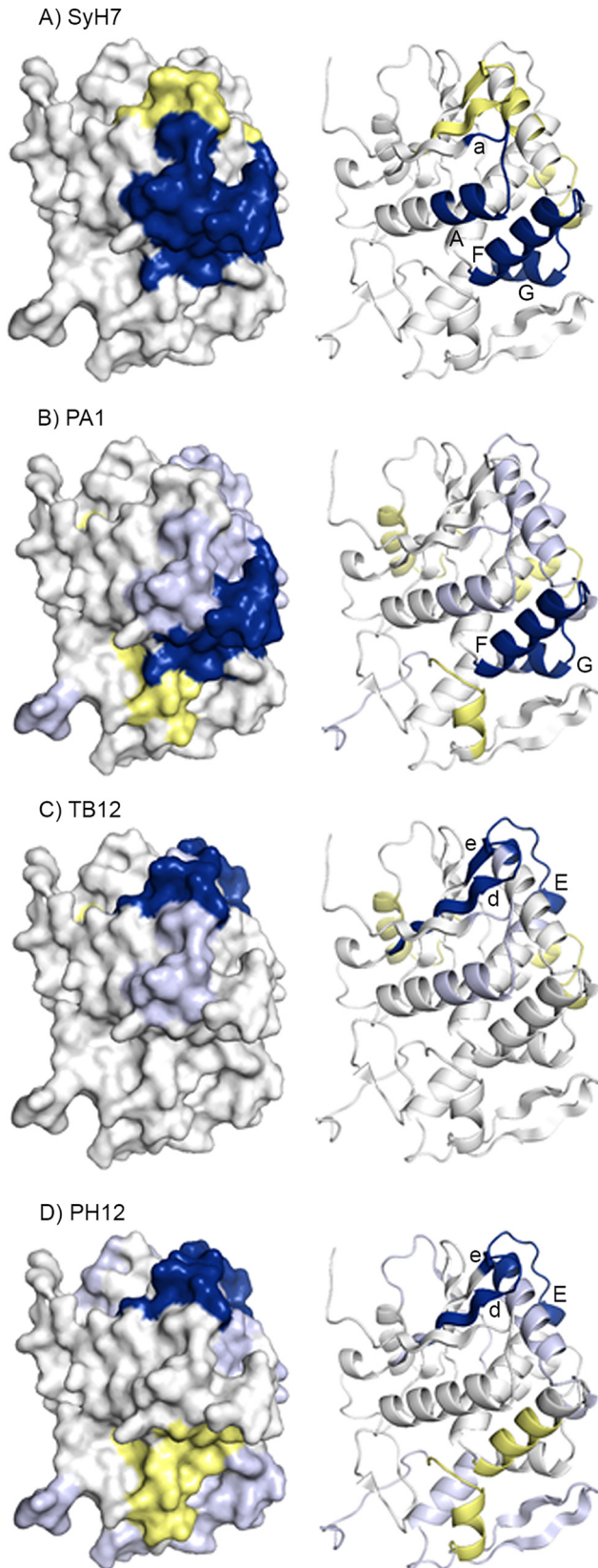
FIG 6 Visual presentation of the core epitopes of SyH7, PA1, TB12, and PH12 on RiVax. HX protection categories, as defined in the Fig. 5 legend, are shown mapped onto the structure of RiVax for (A) SyH7, (B) PA1, (C) TB12, and (D) PH12. The image is color coded according to the Fig. 5 legend. The locations of \beta -strands a, d, and e as well as \alpha -helices A, E, F, and G are indicated.
