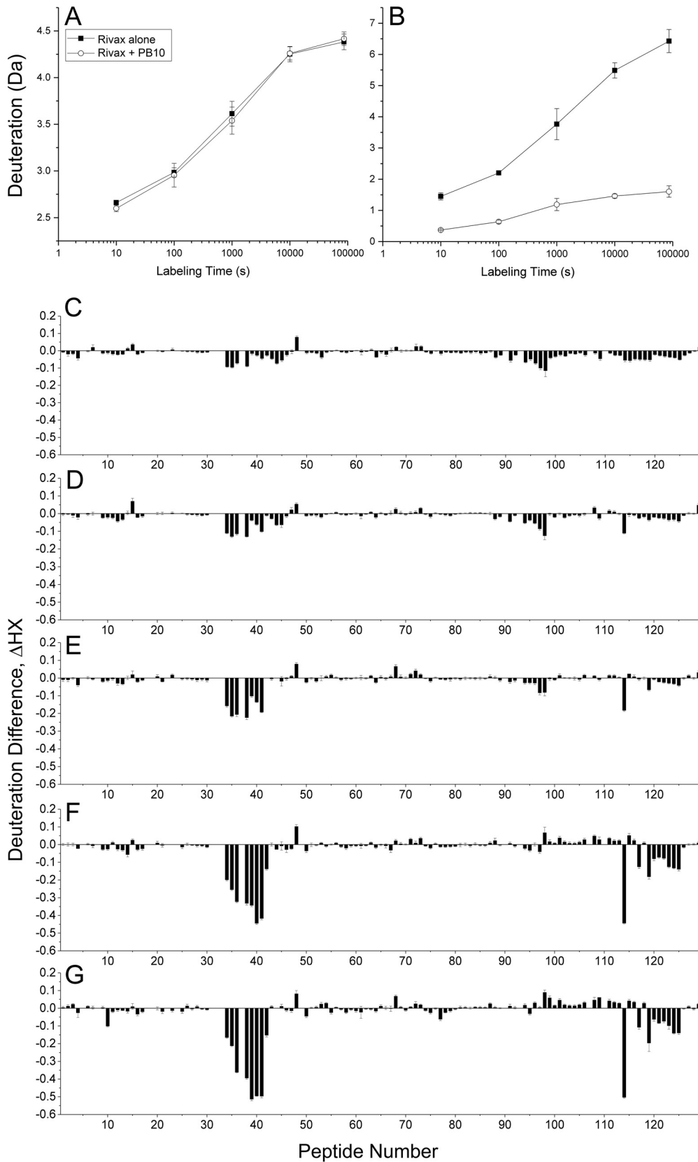
FIG 2 HX-MS analysis of RiVax in the presence of PB10. RiVax was subjected to HX-MS analysis in the absence or presence of MAb PB10. (A and B) HX kinetics of two representative RiVax peptides. Panel A shows peptide 1 (residues 0 to 11), where the rate of HX was unaffected by PB10. Panel B shows peptide 38 (residues 93 to 107), where the rate of HX was significantly reduced by PB10. (C-G) Deuterium difference ( \Delta HX) for various peptides. (Continued on next page)
