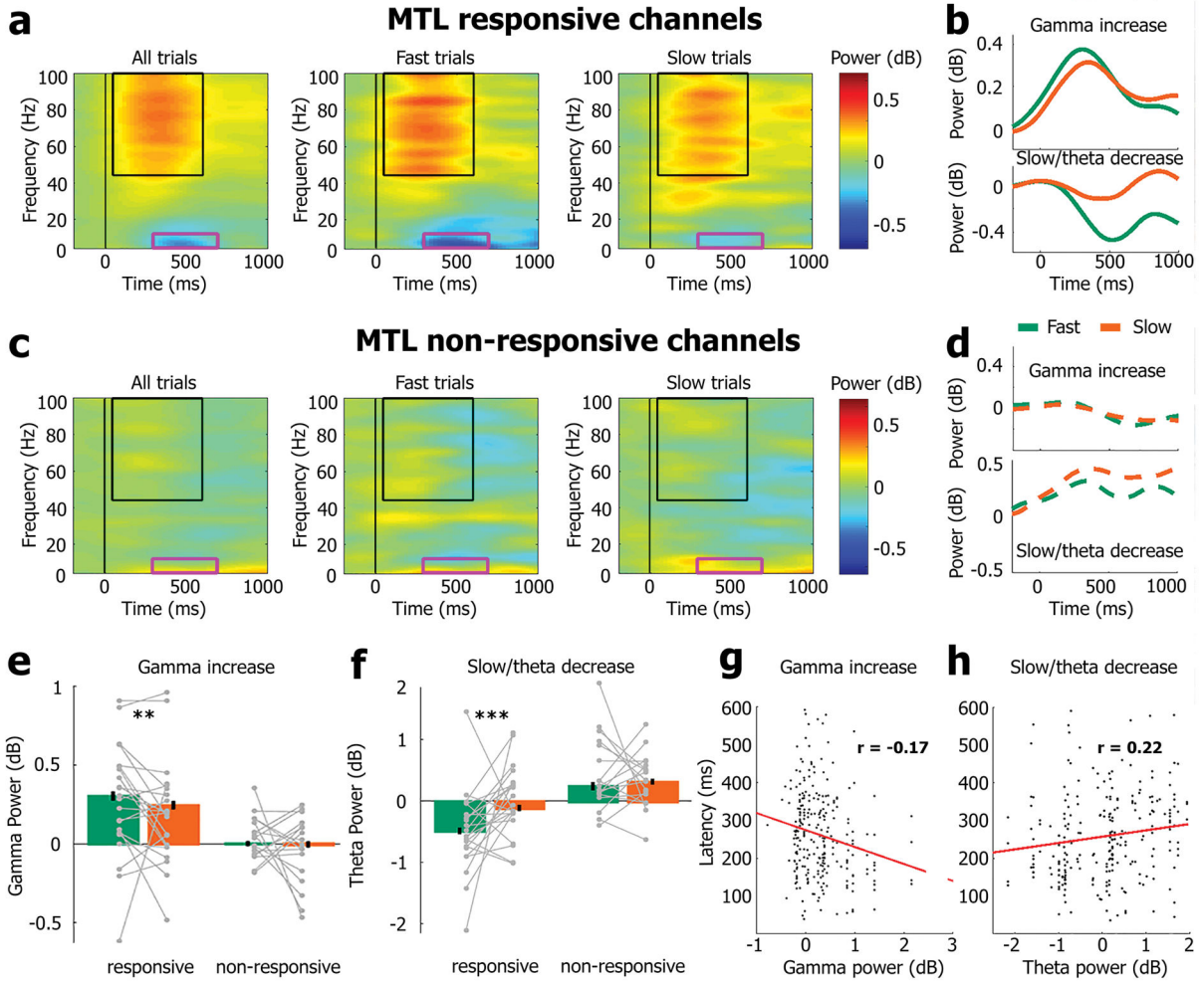
Figure 4. Cognitive lapses are associated with weaker gamma power increase and weaker slow/theta power decrease in MTL LFPs (a) Time-frequency decomposition of induced power changes in local field potentials (LFPs) of MTL responsive channels (n=270 channels in 31 sessions). Columns denote the average power changes for all trials (left), fast trials (lowest RTs, middle), and slow trials (highest RTs, right). In each subpanel, hot and cold colors mark increases and decreases in power, respectively. Black rectangles mark stimulus-induced increase in gamma frequency (>45Hz) power around 50–600ms after stimulus onset. Pink rectangles mark stimulus-induced decreased power in the slow/theta frequency range (2–10Hz) around 300–700ms after stimulus onset. Slow trials are associated with weaker gamma power increase and weaker slow/theta power decrease. (b) Time course of gamma power increase (top) and slow/theta power decrease (bottom) for fast trials (green) vs. slow trials (orange). (c) Same as (a) for neighboring MTL non-responsive channels (n=198 channels in 31 sessions). Note the absence of significant power modulations during the same slow trials in neighboring channels. (d) Same as (b) for neighboring MTL non-responsive channels. (e) Quantification (median) of gamma power increases (45–100Hz; 50–600ms) for responsive (left) and non-responsive MTL channels (right). Asterisks show significant differences (Wilcoxon signed-
