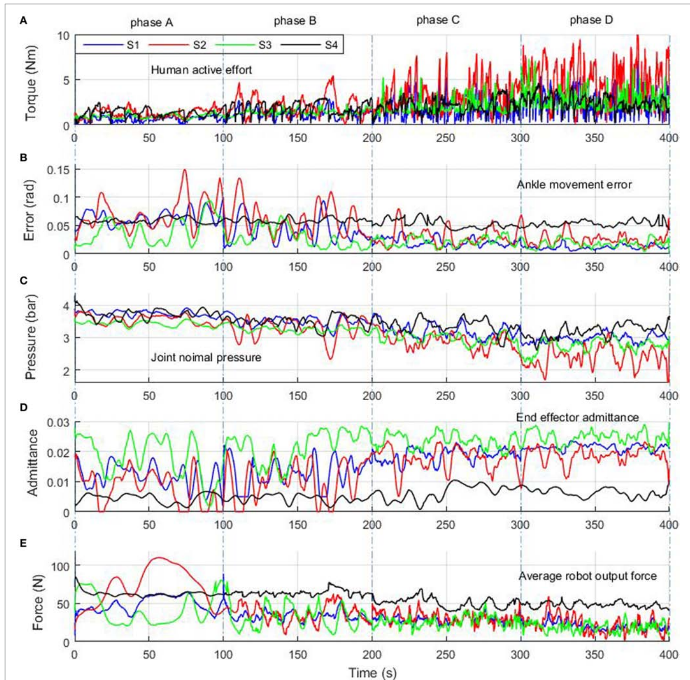
FIGURE 12 | Experiment results of adaptive hierarchical compliance control with four human subjects who were asked to increase active contribution each time from phase A to phase D. Human active effort (A) was calculated using Eq. 20, ankle movement error (B) was obtained from using Eq. 22, joint nominal pressure (C) was regulated based on human participation by Eq. 19, end-effector admittance (D) was adjusted to human movement error (Eq. 21), and average robot force (E) was the mean value of four muscles' pulling forces. Blue, red, green, and dark lines represent the results of S1, S2, S3, and S4, respectively.
