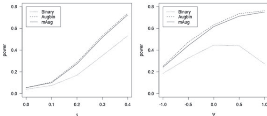
FIGURE 1 Power of the 3 methods for fixed time as the mean log tumour size ratio ( \tau ) varies and as \psi varies at \tau = .35
