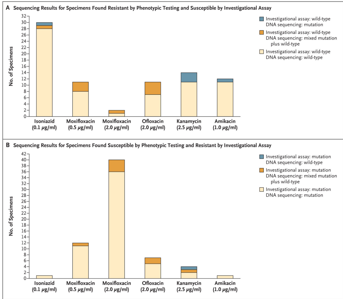
Figure 2. Sequencing Analysis of Isolates with Discrepant Investigational Assay and Phenotypic DST Results
