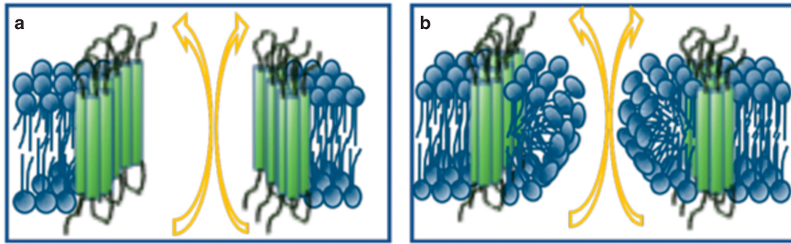
Figure 3 Schematic view of proposed models for structure of membrane pores. (a) Proteinaceous pores consist of BAX/BAK oligomers at the inner rim. (b) Lipid pores are also initiated and stabilized by BAX/BAK oligomerization, but the pore's edge is formed by a monolayer of lipids, allowing hydrophilic proteins to pass the pore
