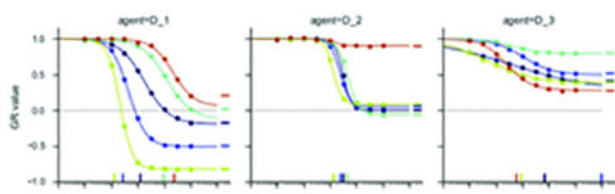
Figure 5. Exemplar Jupyter notebook for evaluating sensitivity metrics (protocol 3) GR values and metrics are calculated using the gr50_tools module (protocol 3, steps 1 and 2). Dose response curves can be plotted and exported as a pdf file.
