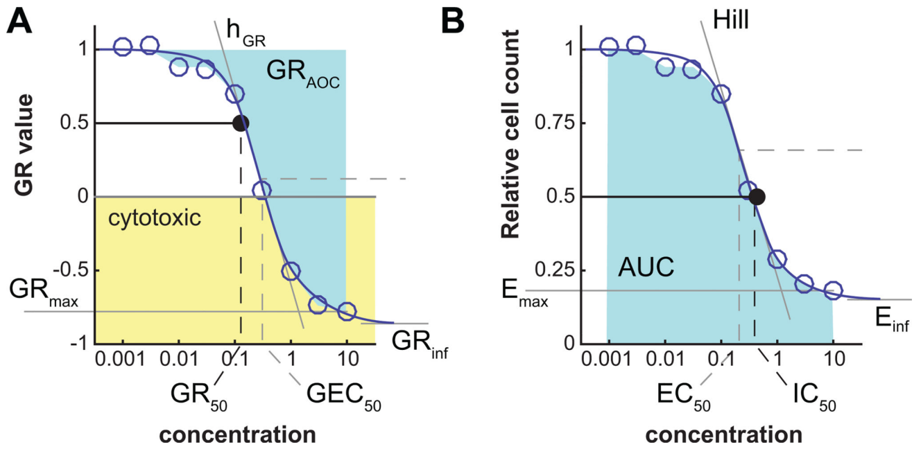
Figure 6. Parameters of a dose-response curve
