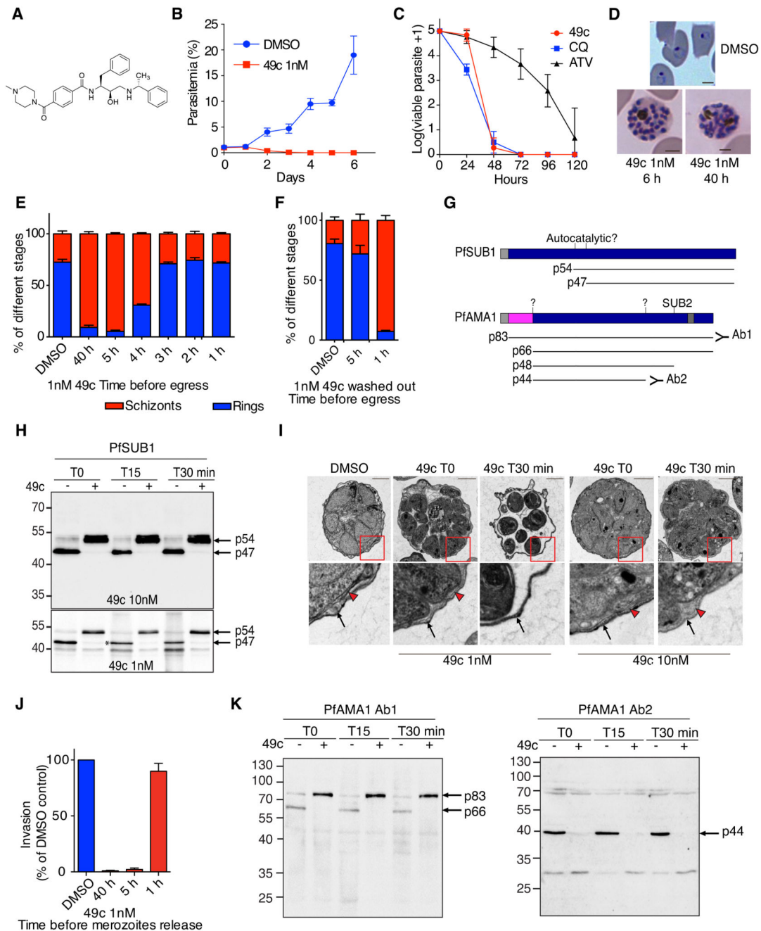
Figure 1. Compound 49c prevents Plasmodium falciparum merozoite egress and invasion. A) Structure of compound 49c. B) WT P. falciparum parasites were treated with 1nM 49c or DMSO, and parasitemia was quantified daily over a six day a period by counting from Giemsa-stained blood smears. Error bars show the SD of three replicates from three independent experiments. C) P. falciparum viability time-course profiles in the presence of 49c (10 nM), chloroquine (CQ, 100 nM), and atovaquone (ATV, 10 nM). D) WT P. falciparum parasites were treated with 1 nM 49c for 6 or 40 hours. DMSO-treated control parasites re-invaded, whereas 49c-treated parasites were blocked at a fully mature schizont
