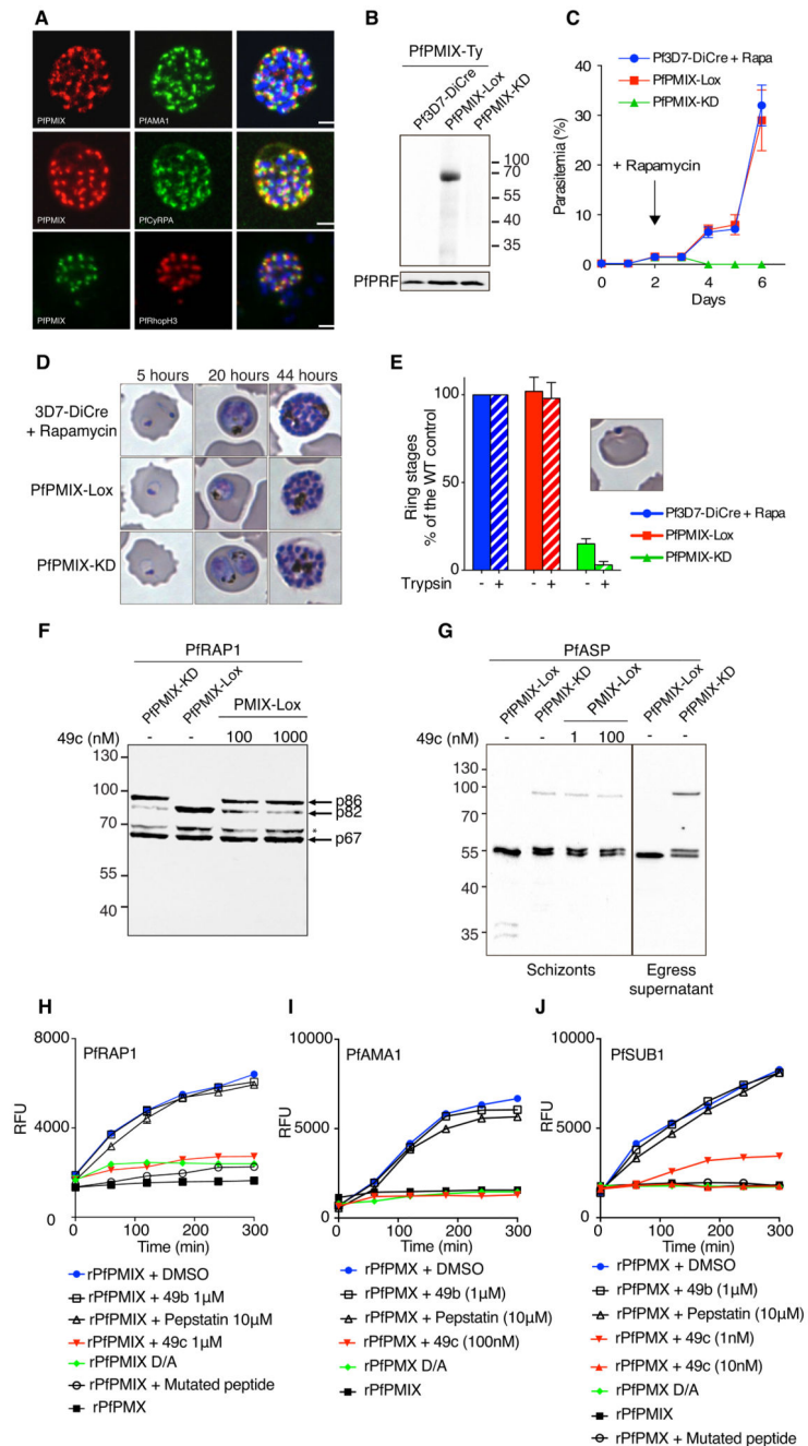
Figure 2. PfPMIX play a critical role in red blood cell invasion
