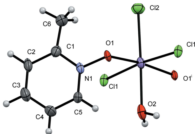
Figure 3 A view of compound II , showing the atom labeling. Displacement ellipsoids are drawn at the 50% probability level. [Symmetry codes: (i) -x - 1, y + \frac{3}{2}, -z + \frac{3}{2} ; (ii) -x, y + \frac{3}{2}, -z + \frac{3}{2} ]
