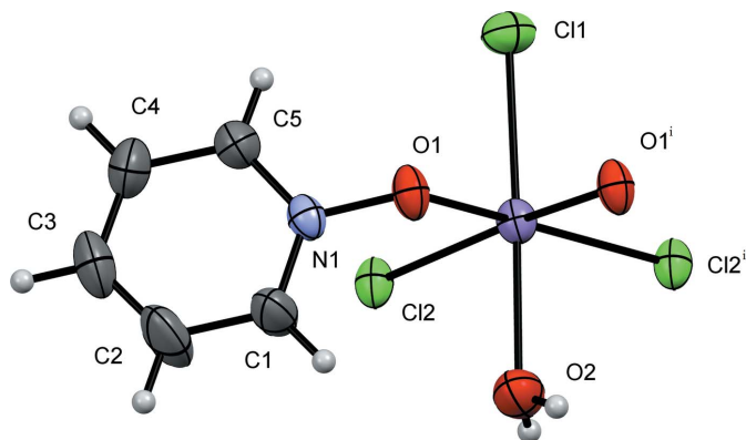
Figure 1 A view of compound I , showing the atom labeling. Displacement ellipsoids are drawn at the 50% probability level. [Symmetry codes: (i) -x + 1, -y + 1, -z + 1 ; (ii) -x, -y + 1, -z + 1 ]
