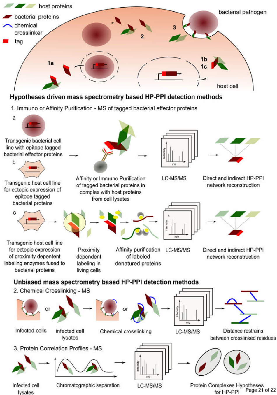
Figure 1. Mass spectrometry based methods for Host-Pathogen Protein-Protein Interactions detections in the context of bacterial infections. AP/IP-MS from epitope tagged bacterial effector proteins (1a) post infections of their host cells enables the identification of physiological HP-PPI. Along with other hypotheses driven methods such as ectopic expressions of tagged bacterial proteins in the host environment (1b and 1c), they can lead to near comprehensive identifications of HP-PPI. However, because they rely on the prior tagging of the proteins of interest, they are limited by the number of proteins that can be cloned and expressed in the
