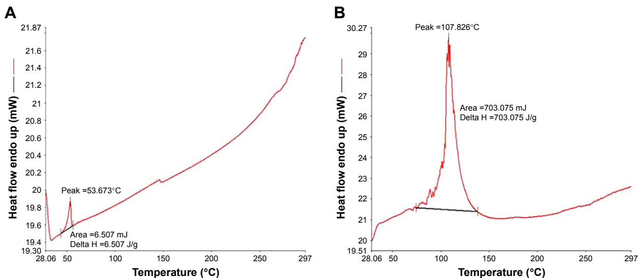
Figure S5 DSC thermograms of (A) NK and (B) optimized-formulation NKNPs.
