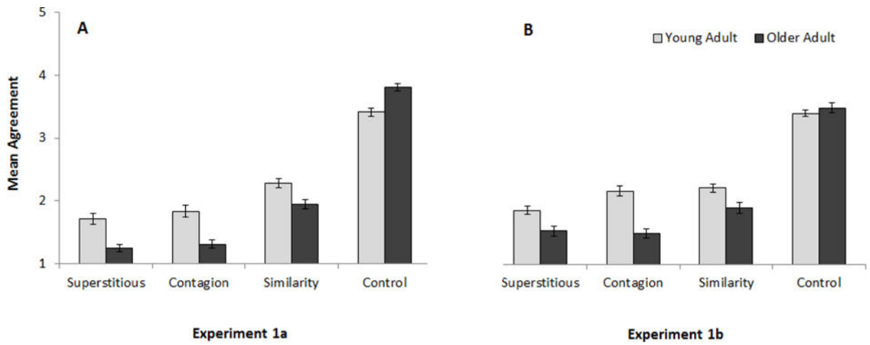
Figure 1. Mean agreement with each item type, graphed as a function of age, in Experiments 1a (A) and 1b (B). Error bars reflect standard error of the mean. Two problematic items are removed from (A) (see text for details).
