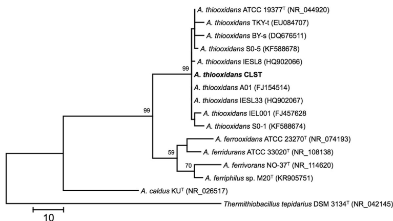
Fig. 1 Phylogenetic tree based on the 16S rRNA gene sequences highlighting the position of Acidithiobacillus thiooxidans strain CLST relative to other type and non-type strains of the genus Acidithiobacillus . The GenBank database accession codes are indicated between brackets. The evolutionary history was inferred by using the Maximum Parsimony and the Subtree-Pruning-Regrafting (SPR) algorithm with search level 1 [52]. The initial trees were obtained by the random addition of sequences. The analysis involved 16 nucleotide sequences and a total of 1307 non-ambiguous positions in the final dataset. Evolutionary analyses were conducted in MEGA version 6.22 [53]. Tree construction used a bootstrapping process repeated 1000 times to generate a majority consensus tree. A sequence from Thermithiobacillus tepidarius was used as outgroup. The tree is drawn to scale, with branch lengths calculated using the average pathway method [53]; the scale bar corresponds to the number of changes over the whole sequence
