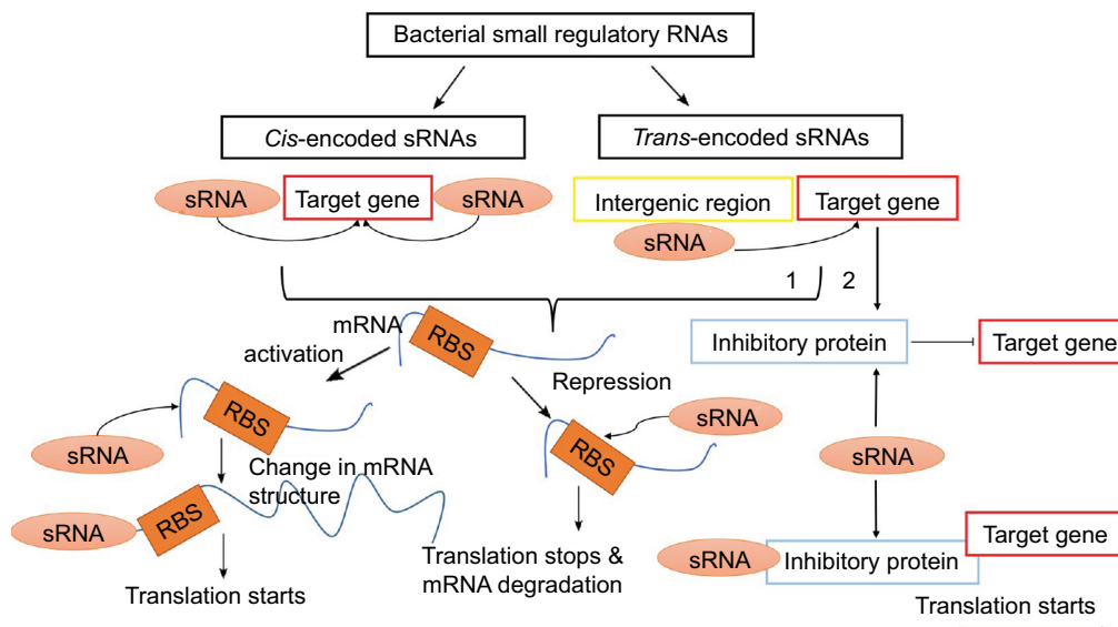
Figure 3 The biological action of small bacterial RNAs. These molecules are classified into cis - and trans -encoded sRNAs. By binding to non-coding region of mRNA or a gene per se, sRNAs either activate or repress the expression of a given protein.
