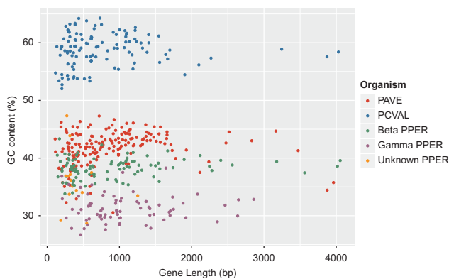
Figure 3 GC versus gene length in the CDS of T. phenacola PPER compared to T. phenacola PAVE and T. princeps PCVAL. The taxonomic origin of the PPER genes is indicated.
