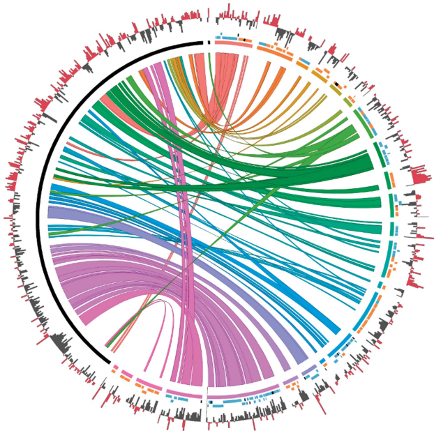
Figure 2 Genome synteny comparison of the two T. phenacola strains already sequenced, PAVE and PPER. Bezier curves highlight regions of synteny shared between both strains. From inner to outer the rings show the PAVE chromosome and plasmid (left) in black, and the PPER contigs (right), each one in a different color; PPER genes in the forward or reverse strand are represented in different colors according to their assigned taxonomic origin, beta (blue), gamma (orange) or unassigned (black); for both genomes, the outer plots represent GC skew, with positive and negative skew depicted in red and gray, respectively.
