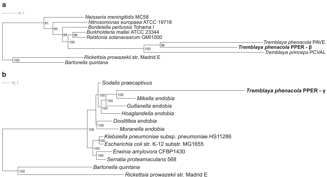
Figure 4 Phylogenomic analysis of T. phenacola PPER. (a) Genes taxonomically affiliated to betaproteobacteria. (b) Genes taxonomically affiliated to gammaproteobacteria. The species used for the analysis are indicated in Supplementary Table S4.
