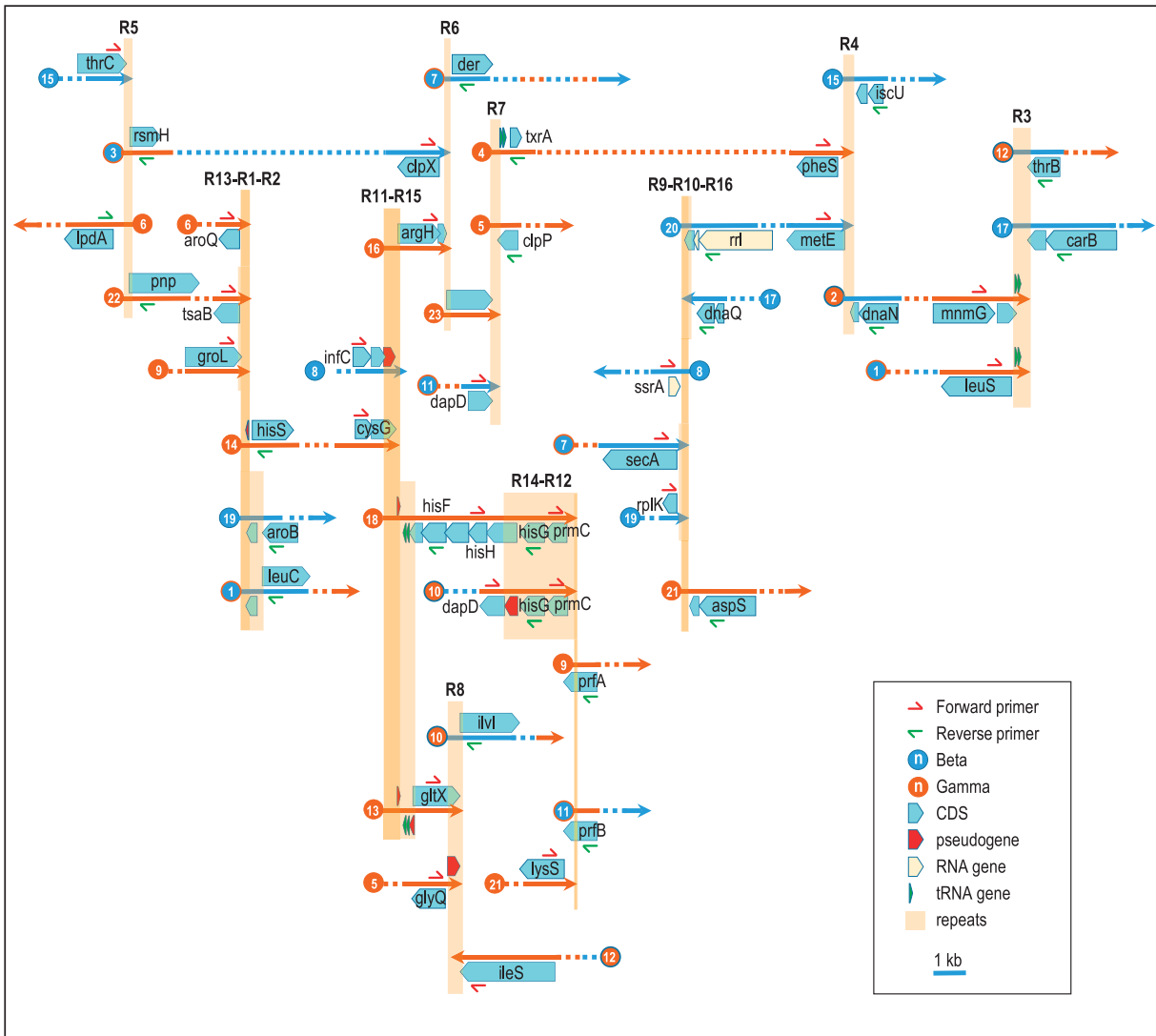
Figure 1 T. phenacola PPER genome representation illustrating all possible joins among contigs. The number of each contig is indicated in a circle at the 5'-end, and the 3'-end is indicated with an arrowhead. The contig lines are colored according to their beta (blue) or gamma (orange) origin. The vertical shadows indicate the end repeats (R1–R16) represented at scale. Genes used for PCR primers designing are shown. Dotted lines followed by an arrowhead indicate that the contig continues in other part of the Figure. When possible, the two ends of the contig are joined by dots, but not at scale. For a description of the repeats, see Table 2.
