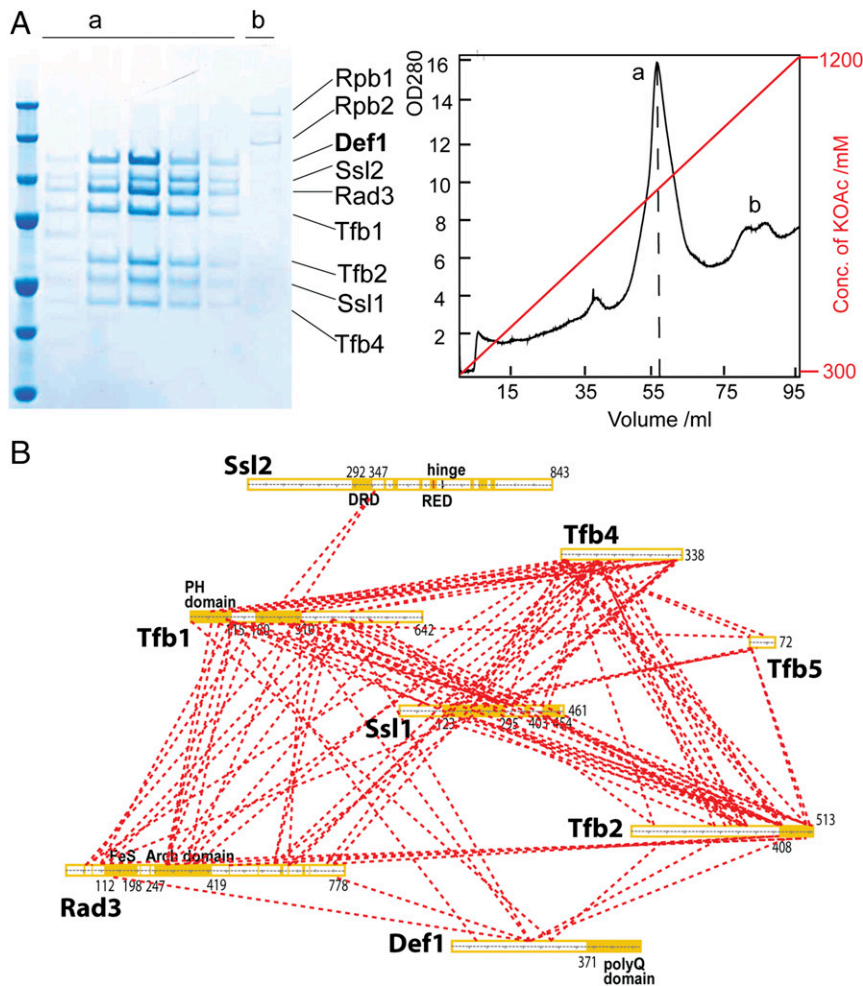
Fig. 1. Coisolation of Def1 with TFIIH from yeast whole-cell extract. (A) TFIIH-Def1 was purified via affinity purification by means of a TAP tag, followed by chromatography on a HiTrapQ column. (Left) SDS/PAGE analysis of the HiTrapQ eluate. (Right) Elution profile of the HiTrapQ eluate. Peaks a and b correspond to Def1-TFIIH and pol II, respectively. (B) Cross-linking map of yeast Def1-TFIIH.
