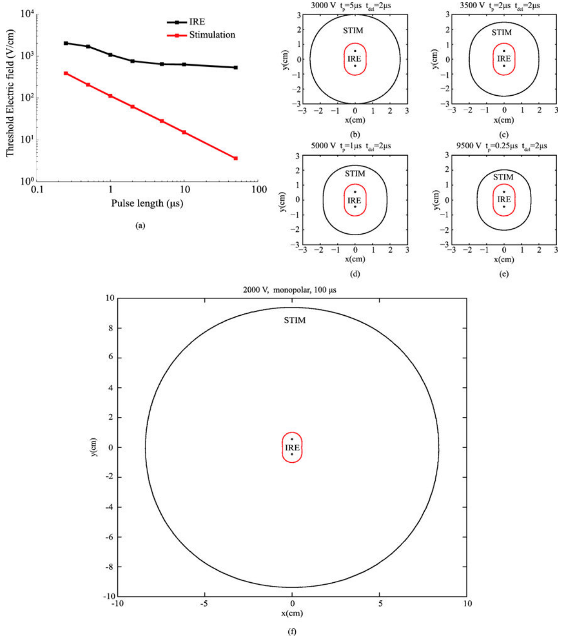
Figure 6. (a) IRE thresholds for PPT8182 cells (from (Sano et al 2015)) and stimulation thresholds for the modeled nerve termination when bursts of bipolar pulses with an energized time 100 μs and an inter-pulse delay of 2 μs are applied. (c)–(f) Simulated areas of ablation (IRE, red boundary) and of nerve termination stimulation (STIM, black boundary) for different pulse lengths and voltages across the needle electrodes. The voltage across the needles was adjusted to obtain a similar ablation area for each pulse length. The represented plane corresponds to the cross-section perpendicular to the electrodes which intersects their centers.
