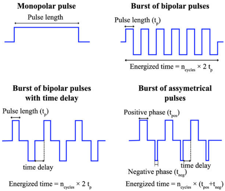
Figure 2. Waveforms considered in the present study.
