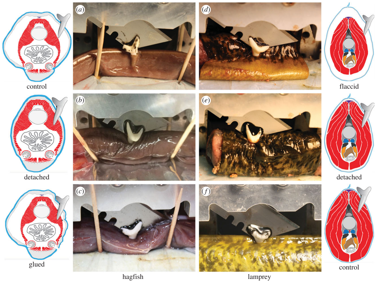
Figure 2. Results of trials in which mako shark teeth were driven into hagfish and lamprey specimens with a spring-driven guillotine. (a) E. stoutii control specimens were punctured every time, but never sustained internal damage. (b) E. stoutii detached specimens were typically punctured through the skin and the underlying muscle. (c) E. stoutii -glued specimens similarly sustained damage to the skin and underlying muscle. (d) P. marinus specimens altered to have a flaccid skin akin to hagfishes were damaged less than unaltered controls. (e) Detached P. marinus specimens sustained damage to both their skin and underlying muscle, which was similar to the results for control P. marinus (f).
