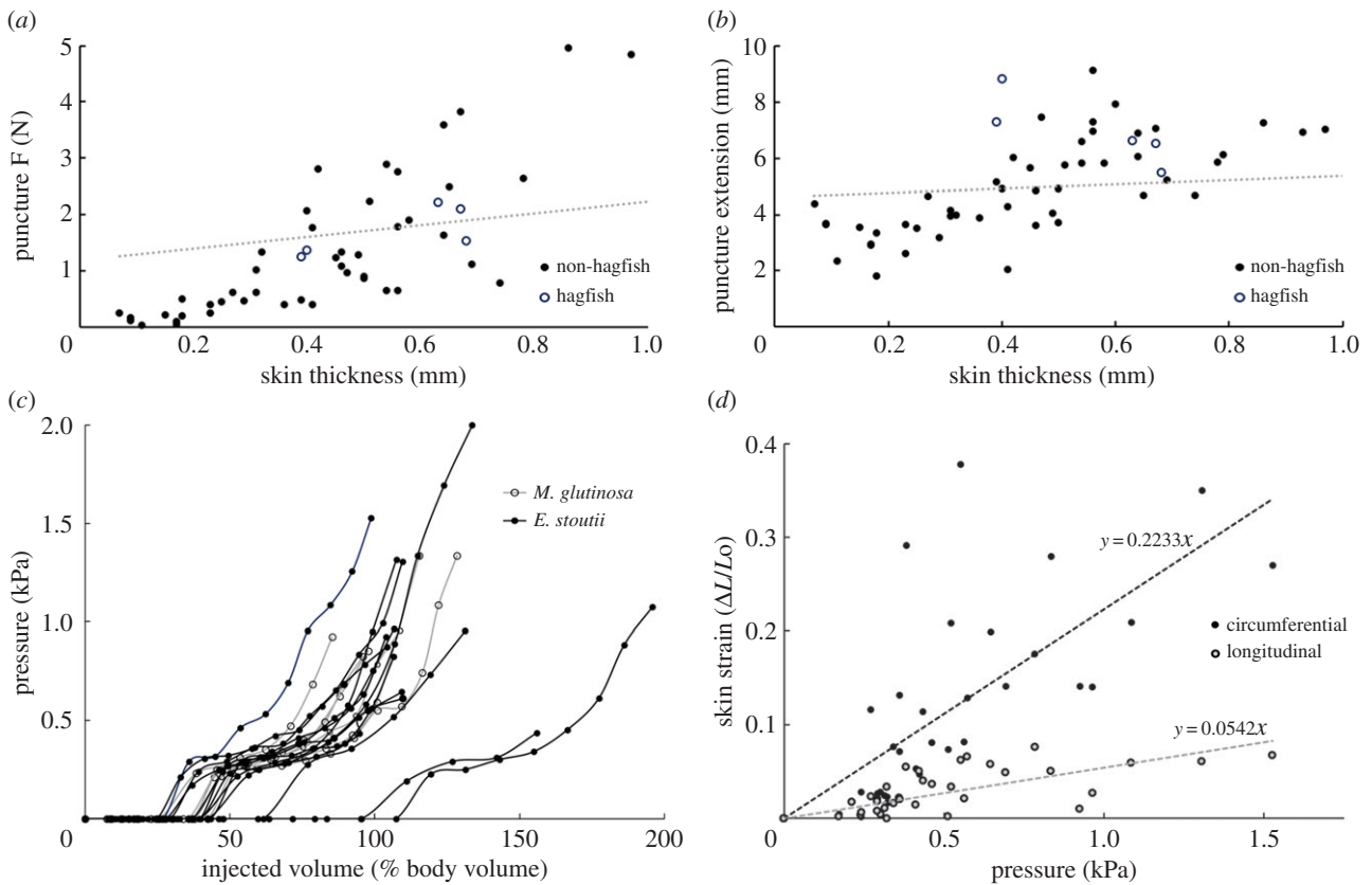
Figure 1. Puncture and inflation of hagfish skin. (a) Load at puncture for E. stoutii skin did not differ significantly ( p = 0.930 ) from values from 21 other fish species when the significant covariate of skin thickness ( p < 0.001 ) was considered, whereas extension at puncture (b) was slightly and significantly higher ( p = 0.012 ). (c) Injection of hagfish Ringer's solution into the SCS and simultaneous measurement of hydrostatic pressure resulted in pressure–volume curves for 13 E. stoutii and six M. glutinosa specimens. The flat part of the inflation curve before pressure starts to rise provides a quantitative measure of an animal's flaccidity or 'slack volume', which in both species was substantial relative to the animal's volume, but did not differ between species ( p = 0.33 ). (d) Skin strain in the longitudinal and circumferential directions as a function of inflation pressure. At higher pressures, circumferential strain was 4.5 times higher than longitudinal strain, suggesting stiffer mechanical properties of the skin in the longitudinal direction.
