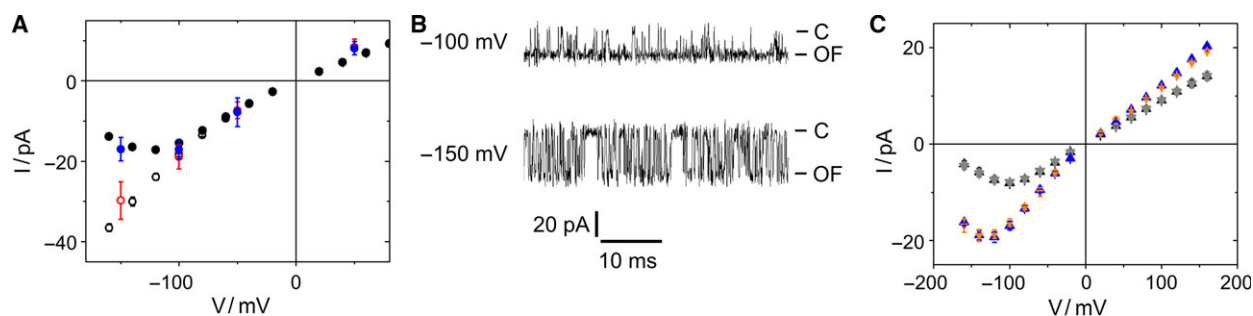
Fig. 4. Reliability of the extended beta distribution fit. (A) I_{app} of Kcv_{NTS} at 1 M KCl as obtained with the 1-kHz filter (black circles) or from filtering the 10-kHz data from Meca-4 chips to ca. 1 kHz by a moving average filter (blue circles). I_{OF} as determined by the extended beta distribution fit with 1-kHz filter [Eqn 1], open black circles, n = 3 and I_{OF} directly measured with the 10-kHz filter (open red circles n = 4 ). (B) Representative current traces of Kcv_{NTS} in 1 M KCl filtered at 10 kHz. Closed channel and I_{OF} are labeled as C and OF, respectively. (C) Current I_{app} measured at 1 kHz for Kcv_{NTS} at 0.1 M (black) and 1.5 M KCl (blue) compared with I_{app} (gray and orange) as calculated from averaging over O-M and O-F gating [Eqn 2]. Mean and standard deviation of 6 and 3 experiments at 0.1 and 1.5 M, respectively.
