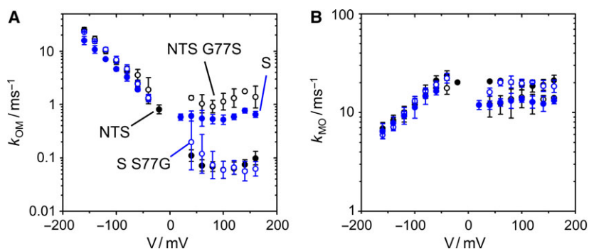
Fig. 6. Two different mechanisms of O-M gating at negative and positive voltages. (A) The two channels with Ser at position 77 at the cytosolic gate ( Kcv_S , filled blue circles, and Kcv_{NTS} G77S, open black circles) have higher values for k_{OM} (channel closing) at positive voltages than those channels with Gly at position 77 ( Kcv_S S77G, open blue circles and Kcv_{NTS} , filled black circles). The voltage dependence at negative voltages is not affected by the mutations, neither is the rate constant of channel opening, k_{MO} (B). N = 3 for Kcv_S , Kcv_S S77G, and Kcv_{NTS} G77S, n = 6 for Kcv_{NTS} wt.
