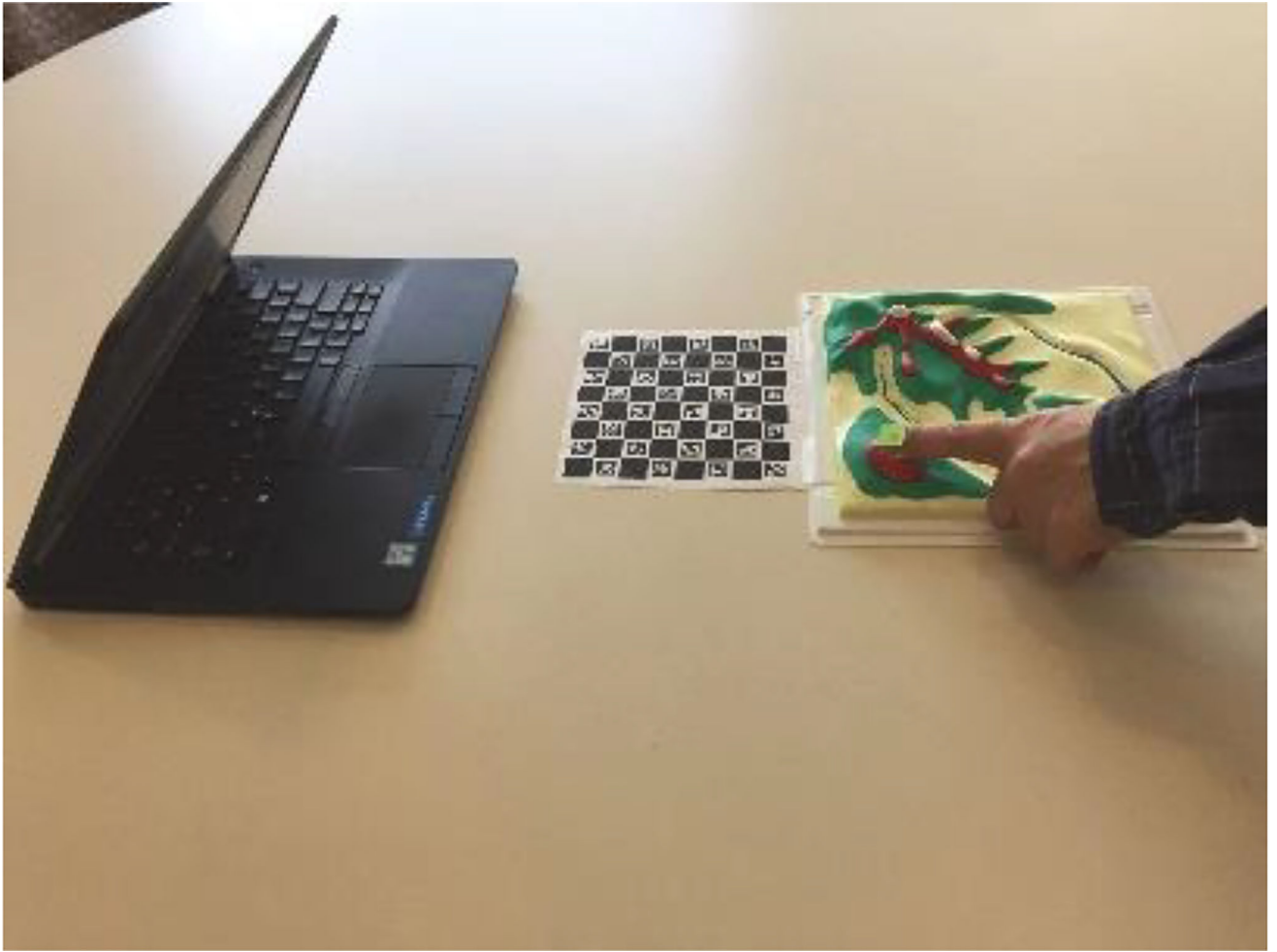
Figure 2. CamIO system shows laptop, object (relief map), fiducial marker board and user pointing to a hotspot.
