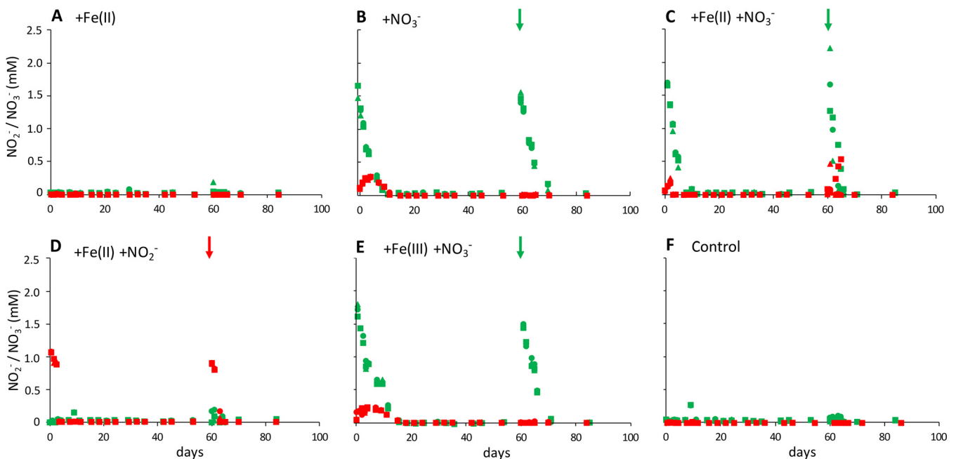
FIG 2 Nitrate (green) and nitrite (red) concentrations in different microcosm setups (triplicates shown with triangle, square, and diamond symbols). After the initial amendment (5 mM each Fe(II) and Fe(III) in addition to 1 mM derived from the sediment, 2 mM each nitrate and nitrite), microcosms were spiked with nitrate or nitrite at day 60 (see arrows). Fe conversion data of the same experiments is shown in Fig. 3.
