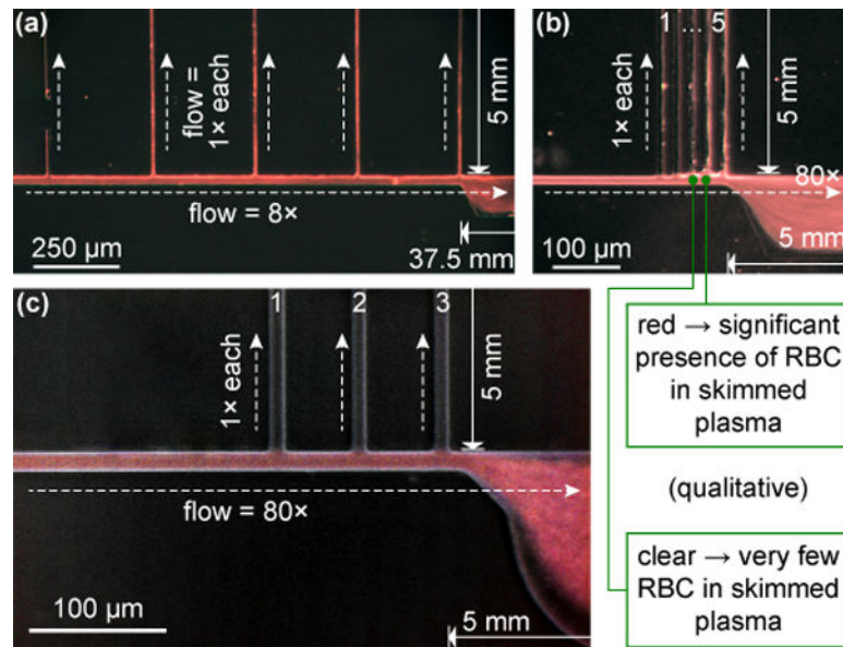
Fig. 2. Plasma skimming microscopy observations for exemplary designs with flow ratios of 8:1 (a) and 80:1 (b–c). The blood inlet is on the left, plasma skimming channels toward the top. Optimized design (c) features enhanced corner definition and only 3 skimming channels.
