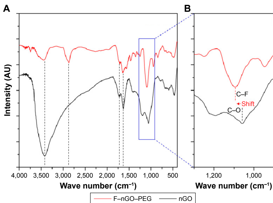
Figure 4 Characterization of nGO and F-nGO-PEG. (A) FT-IR; (B) magnified FT-IR spectra. Abbreviations: FT-IR, Fourier-transform infrared; nGO, nano-graphene oxide; PEG, polyethylene glycol.
