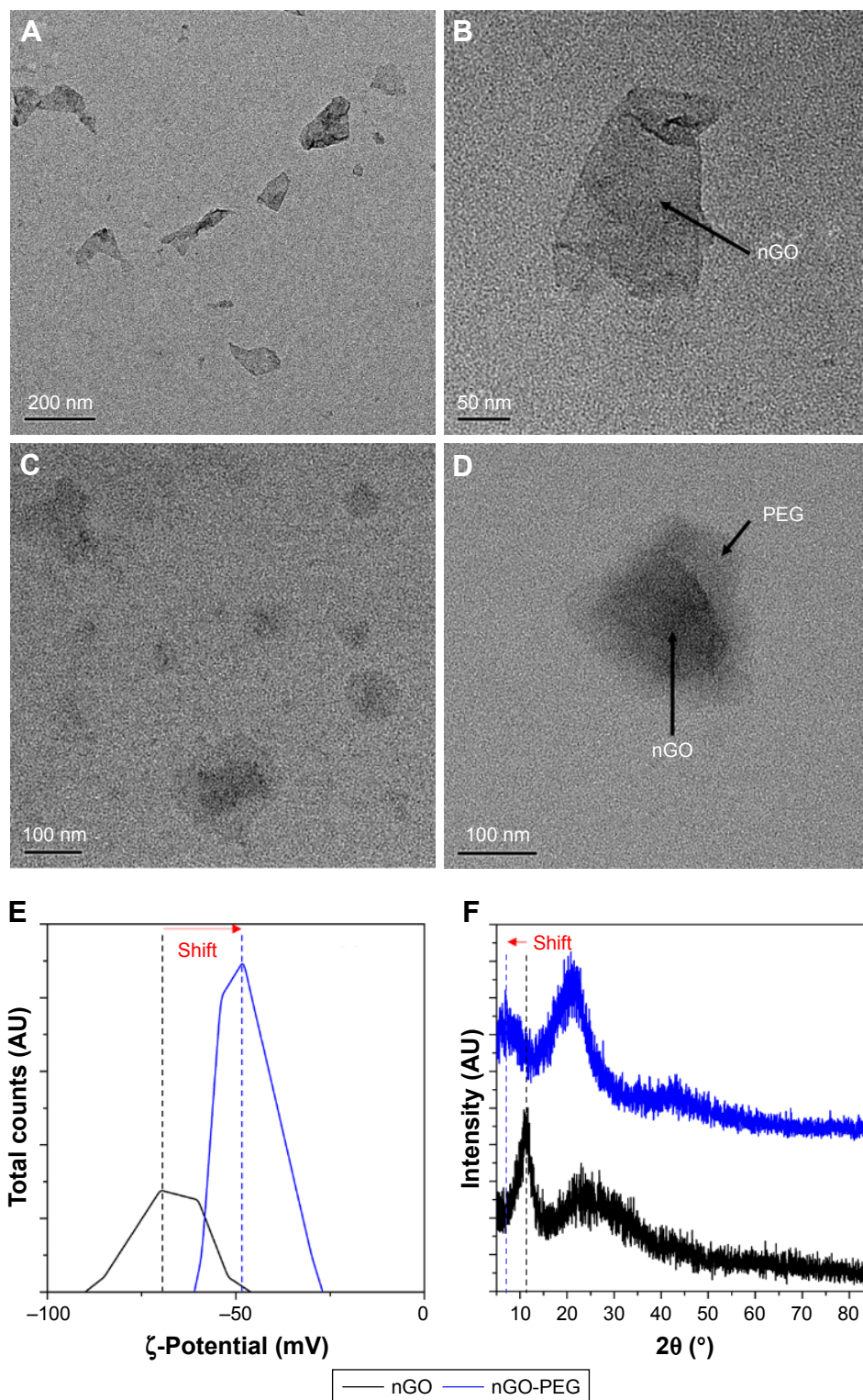
Figure 2 TEM images of (A, B) nGO and (C, D) nGO-PEG; (E) \zeta -potential peak; (F) XRD patterns of nGO and nGO-PEG. Abbreviations: nGO, nano-graphene oxide; PEG, polyethylene glycol; TEM, transmission electron microscopy; XRD, X-ray diffraction.
