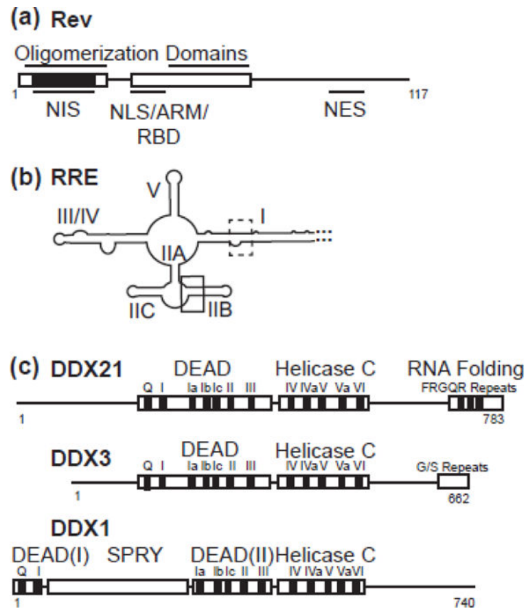
Figure 1. Schematic diagrams of proteins and RNA used in this study. a) Rev, with structured helix-turn helix domains boxed. Oligomerization domains, nuclear export inhibitory signal (nis), nuclear localization signal (NLS), arginine rich motif (ARM), RNA binding domain (RBD) and nuclear export signal (NES) labelled. NIS region has additionally been colored black. b) RRE RNA molecule, with stems I, IIA, IIB, IIC, III/IV, and V labelled. High affinity primary binding site boxed in black, and lower affinity binding site boxed in dotted line. c) DDX21, DDX3 and DDX1 diagrams aligned to DEAD domain and Helicase C domain interface. Accessory domains are labelled.
