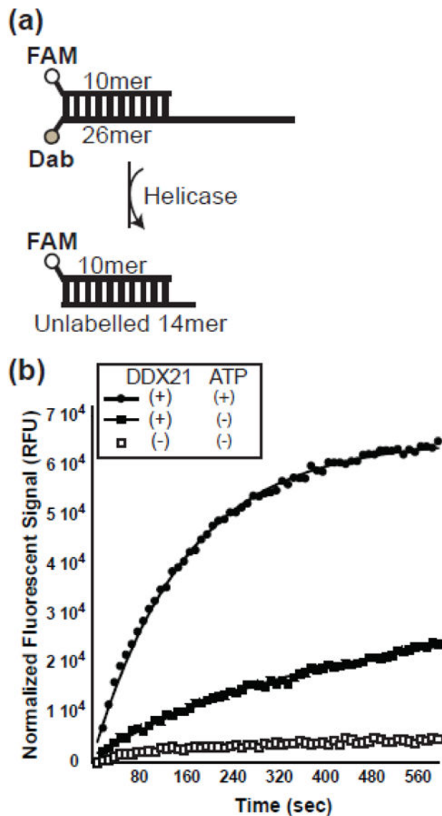
Figure 3. DDX21 helicase activity is stimulated by ATP. a) Schematic diagram of RNA molecules used in helicase assay. A fluorescently labelled RNA 10mer is annealed to a fluorescent quencher 26mer. Once the strands separate, the 10mer reanneals to the excess unlabeled 14mer, resulting in a fluorescent signal. b) Helicase assay results showing a graph of fluorescent intensity over time for RNA dimer alone (open boxes), DDX21 with RNA dimer (closed boxes) and DDX21 with ATP and RNA dimer (closed circles).
