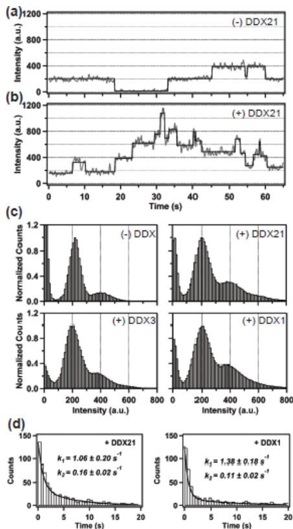
Figure 8. Assembly of Rev on the RRE monitored by single-molecule fluorescence spectroscopy. (a) Rev-RRE assembly in the absence of any DDX protein. Representative time trace (grey) of A555 emission over time, showing individual Rev monomer binding and dissociation events. The emission intensity of a single Rev monomer is ~200 units. The black lines are fits to a hidden Markov model. (b) Rev-RRE assembly in the presence of 150 nM DDX21. Same format as in (a). More Rev monomers assemble on the RRE in the presence of DDX21. (c) Normalized intensity histograms compiled from more than 100 traces, representing individual Rev-RRE stoichiometry states as separate peaks in the absence and presence of 150 nM DDX proteins, as indicated. (d) Dwell time histograms for the first Rev monomer binding to the RRE in the presence of DDX21 (left) and DDX1 (right). Histograms were fitted to a biexponential function, indicated by the solid line. The fitted rate constants and their associated uncertainties are indicated.
