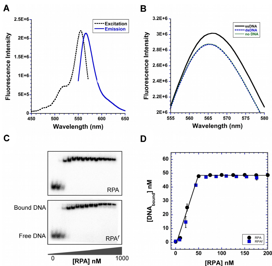
Figure 3. ssDNA binding properties of RPA f . (A) Excitation and emission spectra of RPA f show maximum values at 555 nm ( \lambda_{ex} ) and 566 nm ( \lambda_{em} ). (B) RPA f was excited at 535 nm and emission spectra were recorded in the absence or presence of ssDNA [(dT) 97 ] or plasmid dsDNA. A ~5% increase in fluorescence signal is observed when ssDNA is present in the reaction. (C) Electromobility band shift analysis (EMSA) of RPA WT (top) and RPA f (bottom) binding to 50 nM 32 P-labeled (dT) 35 oligonucleotides show bound and unbound complexes and (D) quantitation of the EMSA data show stoichiometric binding to ssDNA for both RPA and RPA f .
