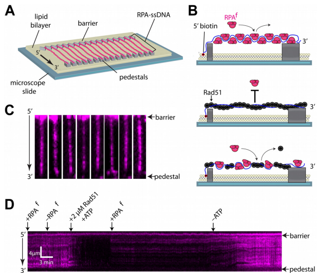
Figure 7. ssDNA curtains to visualize RPA f . (A) Schematic of a RPA f -coated double-tethered ssDNA curtain. (B) Representative examples of individual ssDNA molecules bound by RPA f (shown in magenta). The 5'-biotin tether is oriented at the top of each window that are all 2.7 \times 13.5 \mu\text{m} . (C) Schematic showing the ssDNA curtain experiment time course beginning in the top panel with an RPA f -coated ssDNA molecule. Injecting 2 \mu\text{M} Rad51 displaces RPA f from the ssDNA to form the pre-synaptic filament that is resistant to rebinding of RPA f in the middle panel. Flushing ATP from the system results in spontaneous Rad51 dissociation and the re-binding of RPA f . (D) A representative kymograph of a ssDNA molecule through time. At the start, ssDNA is already coated by RPA f and buffer containing 100 \text{ pM} RPA f is flowing through the chamber at 0.2 \text{ ml/min} . Switching to a buffer lacking RPA f shows that bound RPA f remains stable until the introduction of 2 \mu\text{M} wild type Rad51 when flow is stopped. The loss of RPA f signal is evidence that Rad51 outcompetes the bound RPA f to form a pre-synaptic filament. Resuming flow with buffer containing 100 \text{ pM} RPA f and 2 \text{ mM} ATP shows the ssDNA remains dark as RPA f cannot displace Rad51. However, switching to buffer with 100 \text{ pM} RPA f and no ATP shows assembly and disassembly of a wild type Rad51 filament on an RPA f -coated ssDNA molecule.
