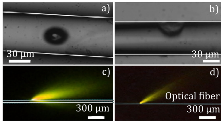
Fig. 7. a) 5 \mu\text{m} opening hole on the buffer layer of a 65 \mu\text{m} fiber to expose the silica cladding; b) Crater-shaped window created by buffer HF etching through the hole; c) Wide side-firing light profile after buffer HF etching; d) Narrow side-firing light profile after gold coating. Fiber samples were coupled with green laser light (532 nm) and immersed in the R6G solution. White lines are used to outline the fiber. White arrows indicate the light propagation direction in the fiber.
