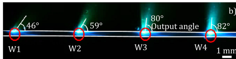
Fig. 4. a) Side window's dimension and firing angle fabricated at different laser power; b) Fluorescent profile of side-firing light from an optical fiber with four windows in acridine orange solution. Red circles show the position of each side window. The white arrow indicates the light direction in the fiber. The distance between each window is 8 mm.
