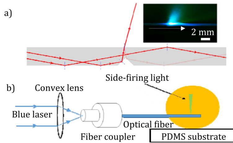
Fig. 2. a) The crater-shaped window causes the input light incident angle to exceed the TIR critical angle, thus part of the input light refracts through the fiber; top right: side-firing light profile in acridine orange solution. The white arrow indicates the direction of blue laser light (473 nm) inside the fiber; b) Optical setup used to take fluorescent profile image of side-firing light from the window.
