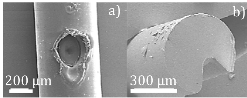
Fig. 1. SEM image of light window fabricated by 50 W CW laser. a) Top view of side window with buffer and cladding layers intact; b) Cross section of the side window without the buffer and cladding layers.
