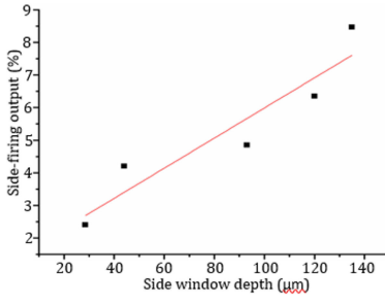
Fig. 5. Side-firing output from windows at different depths. The side window depth was controlled by tuning the power of the ablating CW laser.
