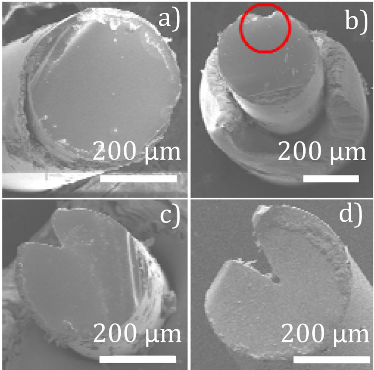
Fig. 3. Cross section of the fiber core after ablation with different laser powers. The window increased in both width and depth when ablated with increasing laser power. a) Laser power of 10 W, no visible change on the fiber core; b) 20 W, a small dent appears on the core (red circle); c) at 30 W, laser started ablating a large portion of the core; d) Deeper window at 40 W.
