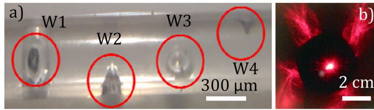
Fig. 6. a) Four windows W1–W4 (red circles) positioned along the fiber axis at orientations of 0°, 90°, 180°, 270° difference; b) The 3D light configuration from these four windows. The fiber was coupled with a HeNe laser ( \lambda = 633 \text{ nm} ) and placed inside a conical frustum to image the side-firing light profile.
