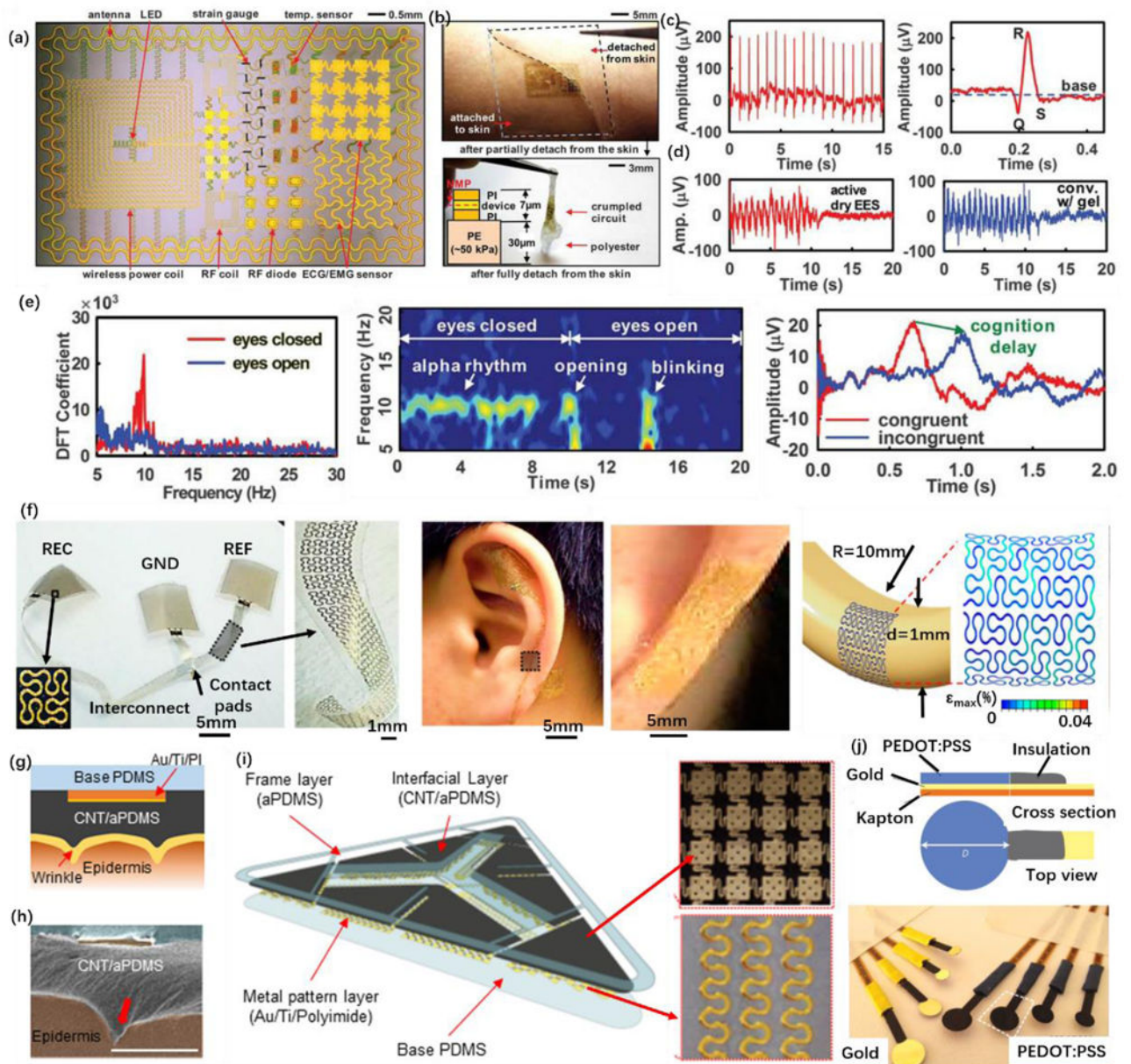
Figure 12. Demonstration of dry epidermal electrodes. (a) An electronics platform with multifunctionality and matched physical properties to skin. 116 (b) The device conformally attached to the skin through van der Waals forces with negligible mass or mechanical loading on the skin. (c) ECG signals measured with an active epidermal electronic device shown in (b), showing a clear physiological signal corresponding to a single heartbeat (right) and (d) EMG measurements showing the comparison with that collected using conventional gel electrodes. (e) EEG measurements using a passive electronic device, including discrete Fourier transform coefficient of EEG alpha rhythms at \sim 10 Hz (left), the spectrogram of the alpha rhythm corresponding to the eyes close and open, and demonstration of Stroop effects in EEG. (f) Epidermal electronics with fractal architectures, showing devices laminated on
