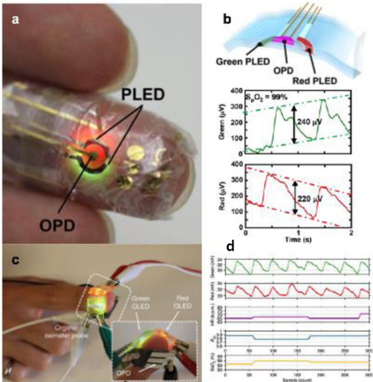
Figure 14. a) Organic pulse oximeter based reflectance scheme. (b) layout of the system with concentric LED's and circular photodiode with resulting signal output. (c) Organic Transmission based oximeter, with subsequent resulting raw data and signal extraction (d).
