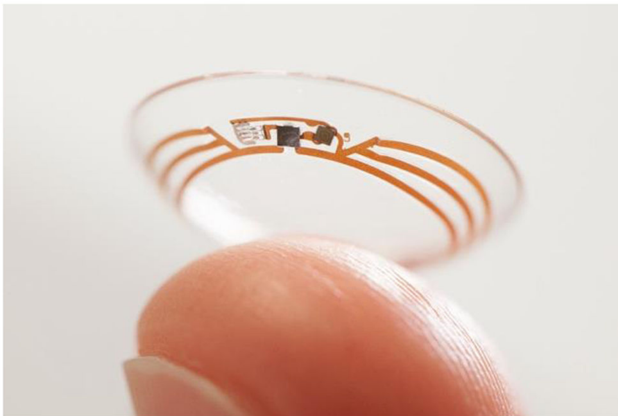
Figure 19. The contact lens sensor that was under co-development by Google and Novartis (effort ceased) measures glucose concentration in tears using a miniaturized electrochemical glucose sensor and a wireless chip and antenna ring. Copyright 2014, Google X.
