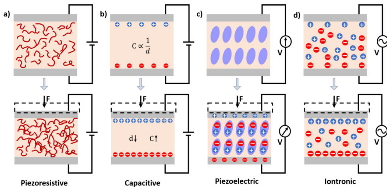
Figure 5. Schematics illustrating the different modalities of mechanical sensors. a) Piezoresistivity b) Capacitance c) Piezoelectricity 190 d) Iontronic.
