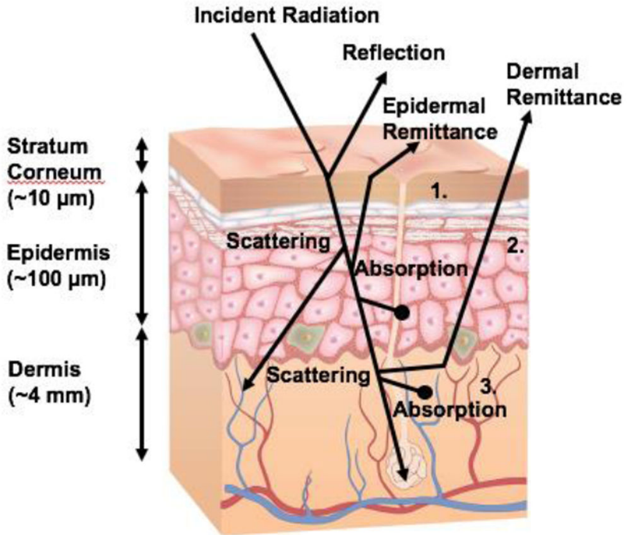
Figure 4. Schematic diagram of optical pathways in skin. Species largely responsible for absorption and scattering in the skin are: keratinized squamous cells (1) and large melanin aggregates (2). The vascularized dermis (3) includes absorbers such as oxygenated and deoxygenated hemoglobin, carotene and bilirubin. Scattering occurs on collagen fibrils and bundles.
