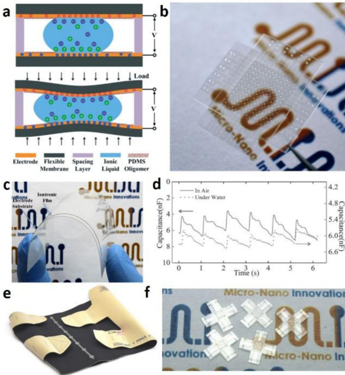
Figure 10. (a) Iontronic droplet sensor operation principle. (b) Photo of an iontronic microdroplet sensing array. (c) Photo of a flexible ionic gel film on electrode substrate. (d) Real-time pulse pressure waveforms in the dry and underwater environments. (e) Photo of a commercial inelastic leggings integrated with the iontronic flexible sensing array. (f) Prototypes of the microfluidic tactile sensors for three-dimensional force measurements.
