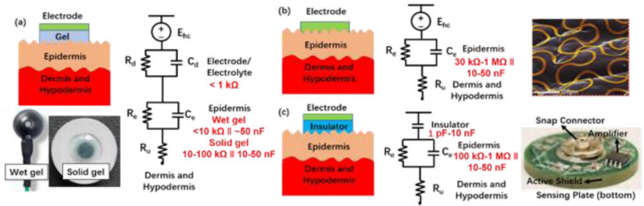
Figure 3. Equivalent circuit models of electrode-skin interfaces for different electrode designs. (a) Gel electrodes, including wet and solid forms (Disposable Deep EEG Cup Electrode, Rhythmlink; ECG Electrode H1354LG, Kendall). (b) Dry contact electrodes. 61 (c) Dry capacitive (non-contact) electrodes. 51
