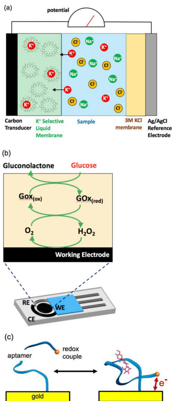
Figure 16. Examples of continuous electrochemical sensing modalities including (a) ion-selective/potentiometric, (b) enzymatic/amperometric where RE is reference electrode, CE is counter electrode, and WE is the working electrode, and (c) simple representation of aptamer-based sensing. Only (a) and (b) have been demonstrated in non-invasive wearable sensors while (c) has only been demonstrated in invasive sensing formats (in circulating blood 165 ). Generally the detection ranges are mM's for (a), down to \mu\text{M} 's for (b) and down to nM's for (c).
