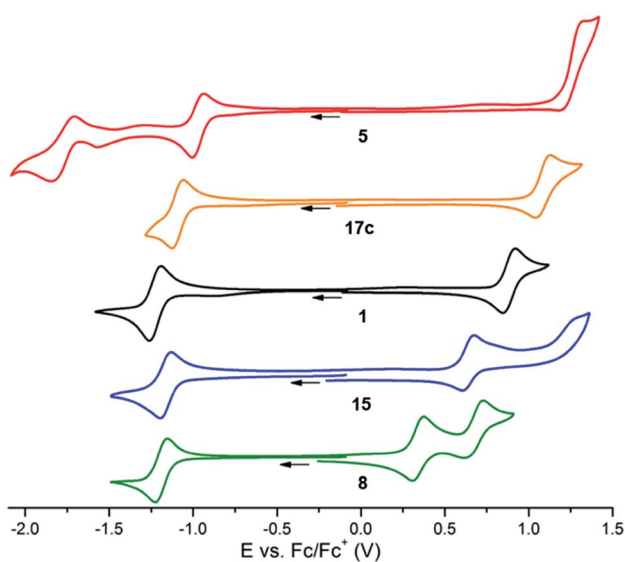
Fig. 3 Voltammograms of acetonitrile ( [\text{TBA}][\text{PF}_6] 10^{-1} M) solutions of 5 (red), 17c (orange), 1 (black), 15 (blue) and 8 (green) ( 10^{-3} M) recorded at a Pt working electrode ( \nu = 0.1 V \text{s}^{-1} ).
