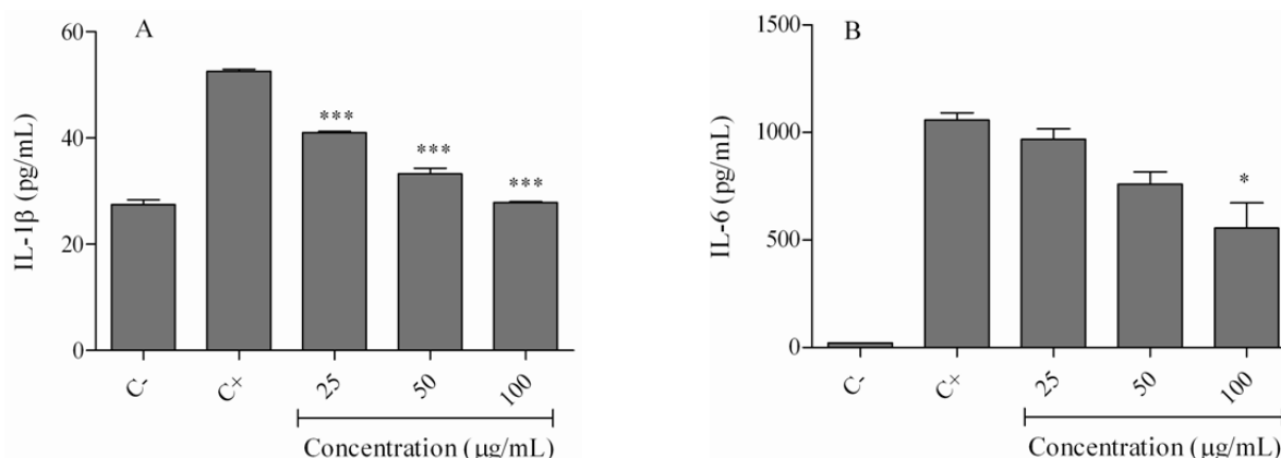
Fig. 5. Effects of the Echium amoenum hexane extract on lipopolysaccharide-induced inflammatory cytokine levels. Cells were treated with 25-100 \mu\text{g/mL} of the hexane extract in the presence of lipopolysaccharide for 24 h. (A) IL-1 \beta , and (B) IL-6 (B) cytokine levels were determined using ELISA. (C-) negative control values were obtained in the absence of lipopolysaccharide and the extract; (C+) positive control was lipopolysaccharide-only treated cells. * P < 0.05 , *** P < 0.001 vs positive control; IL, interleukin.
